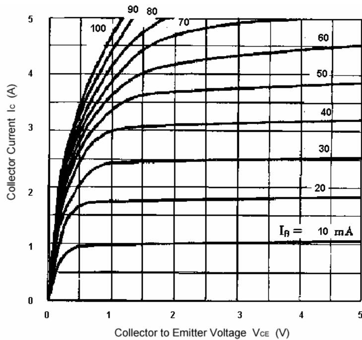
Fig.4 Static Characteristic
