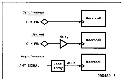
Figure 3. Clocking Modes
