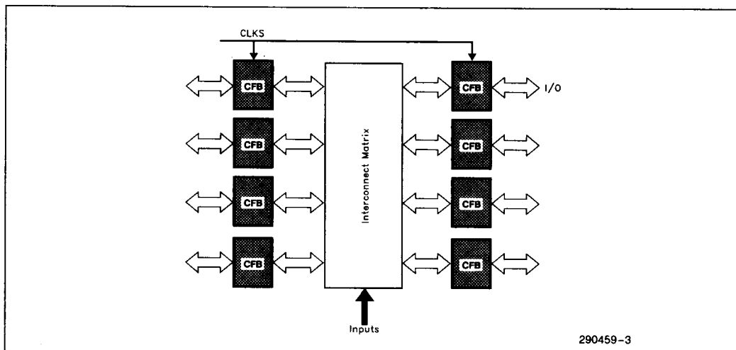
Figure 1. Interconnect Matrix
