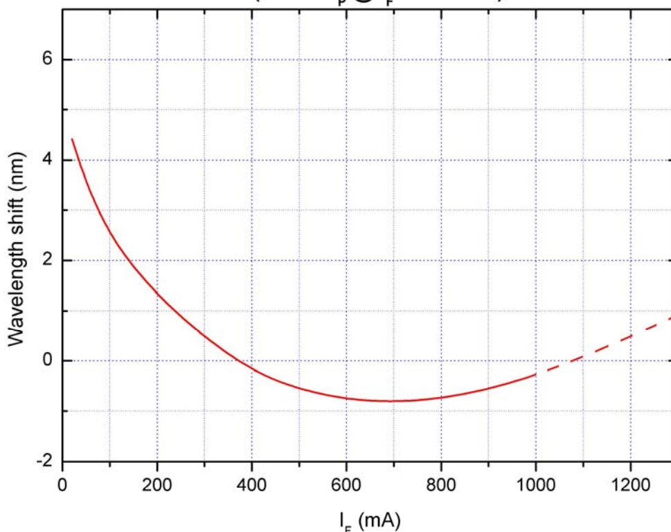
Typical wavelength shift vs. forward current (rel. to \lambda_p @ I_F = 350 \text{ mA} )
