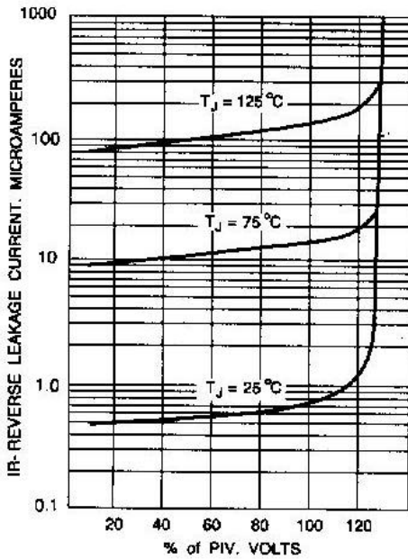
Fig. 3-TYPICAL REVERSE CHARACTERISTICS
