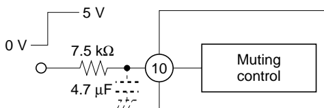
Figure 2 How to use Muting Circuit
