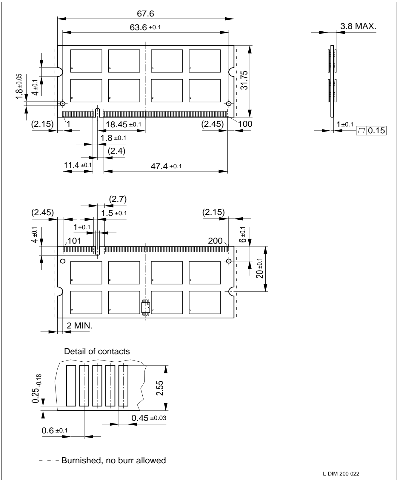
Figure 3 Package Outlines – DDR-SDRAM SO-DIMM HYS64D64020[H/G]BDL-6-C
