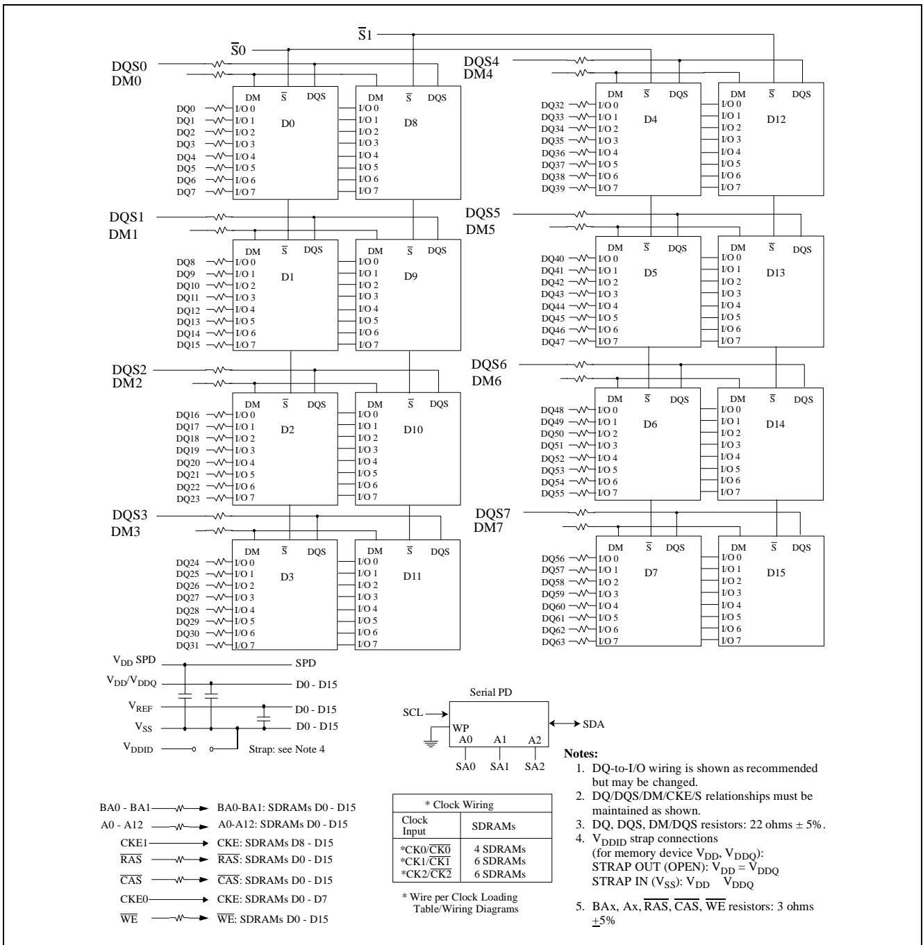
Figure 2 Block Diagram - Two Ranks 64M x 64 DDR SDRAM SO-DIMM HYS64D64020[H/G]BDL-6-C
