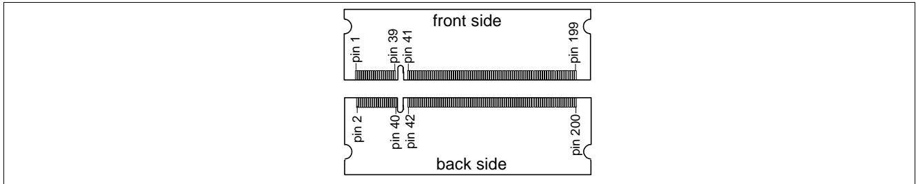
Figure 1 Pin Configuration
