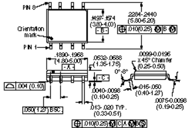
8-Lead SOP outline dimensions Narrow body .150 (All dimensions per JEDEC No. MS-012-AA, Issue C) Dimensions in ( ) are in mm. Unless Otherwise Noted: xxx = \pm 0.010 (xxx = \pm 0.25 ) xx = \pm 0.02 (x = \pm 0.5 )
