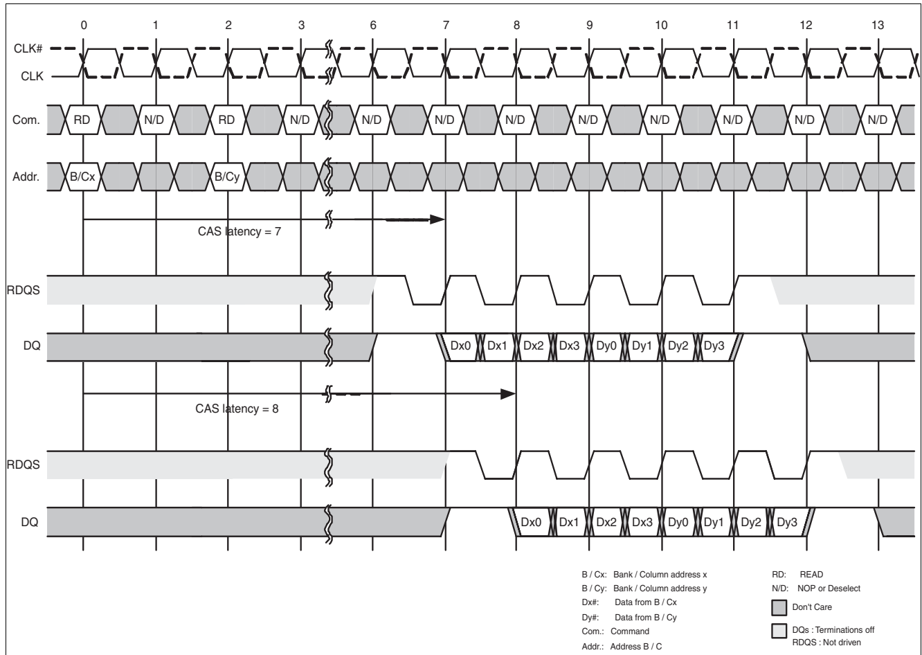
Figure 38 Gapless Consecutive Read Bursts
