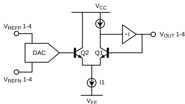
Figure 4. Simplified Block Diagram
