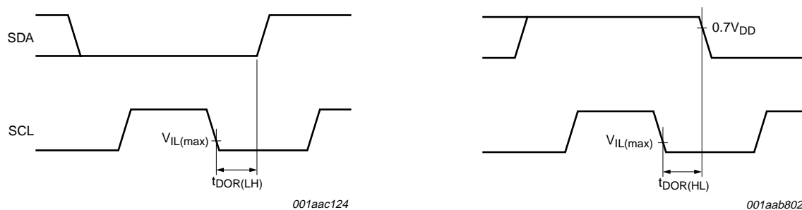
Fig 41. Data output reaction time of the IC
