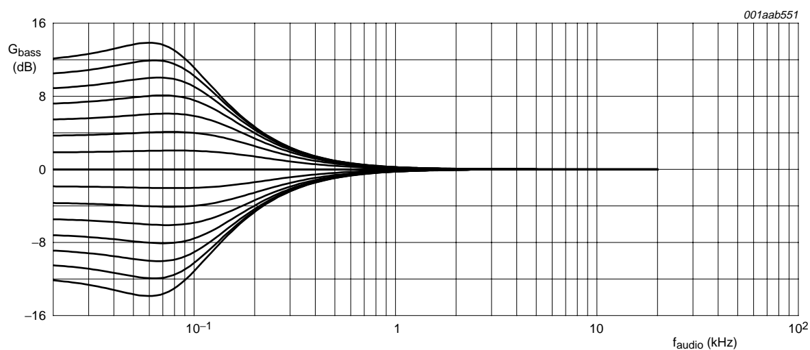
Fig 38. Bass amplitude control characteristics; bass frequency (BAF) = 60 Hz
