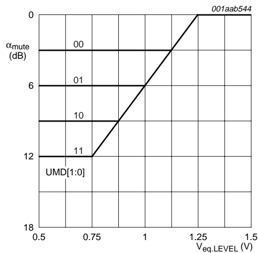
Fig 30. USN soft mute depth settings; USN detector
