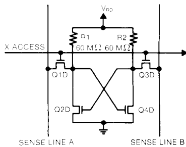
Figure 4. MEMORY CELL
