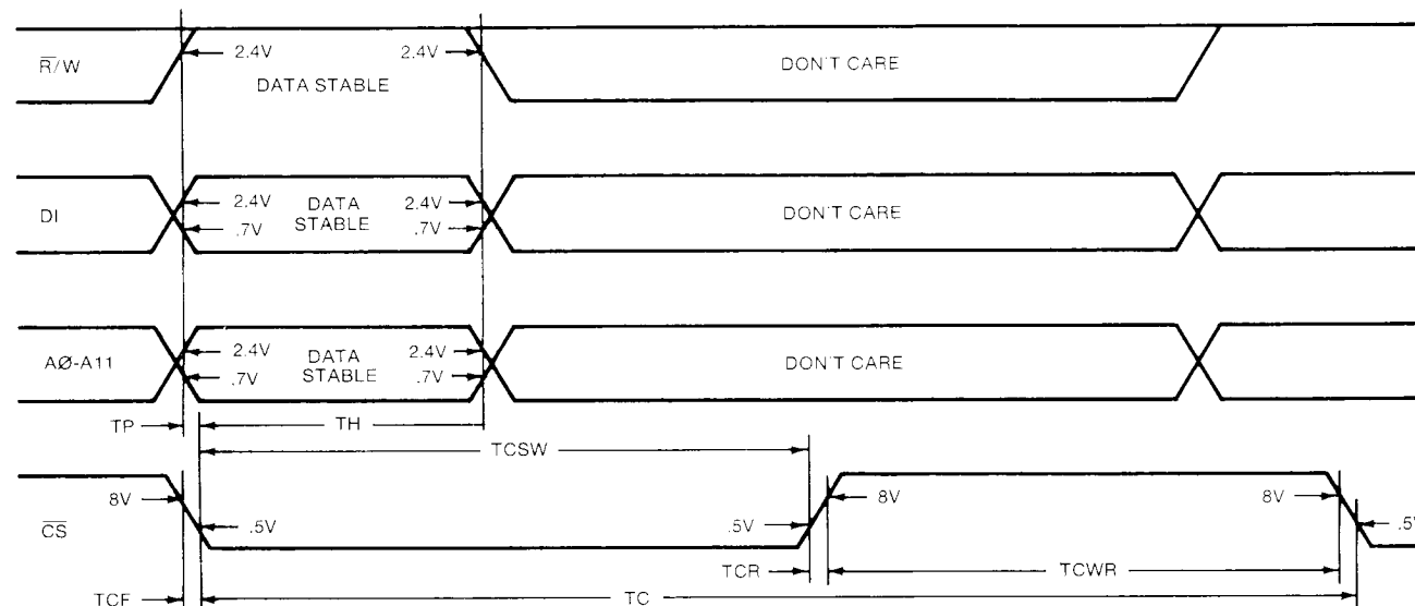
Figure 2 – WRITE CYCLE
