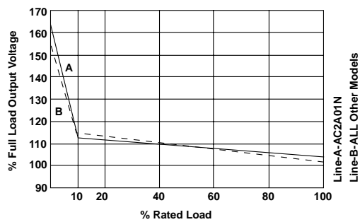
Typical Load Regulation
