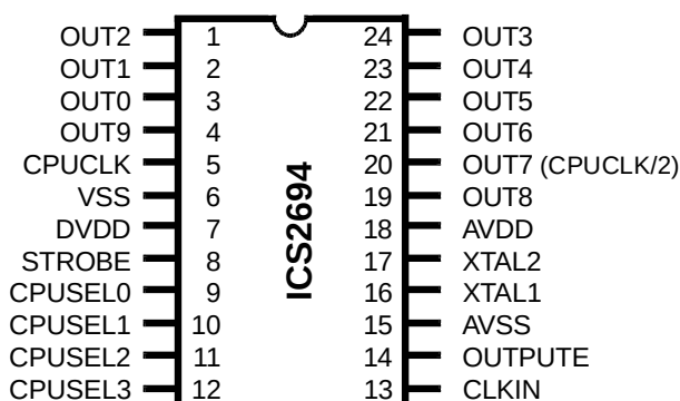
24-Pin DIP or SOIC
