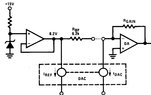
FIGURE 3. Bipolar Configuration
