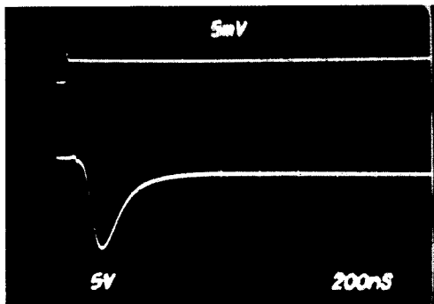
FIGURE 2. Voltage Mode Settling Time—1 LSB Change
