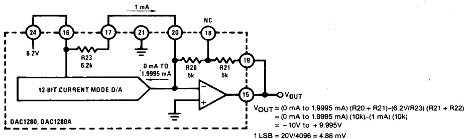
FIGURE 5. ±10V Bipolar Operation
