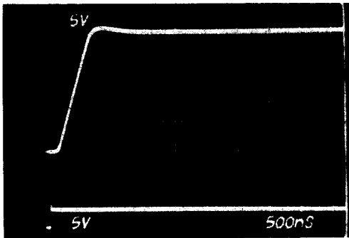
FIGURE 1. Voltage Mode Settling Time—FSR Change
