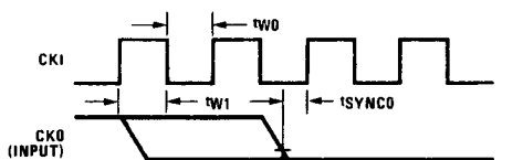
FIGURE 3A. Synchronization Timing
