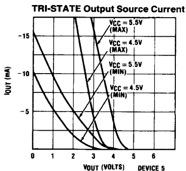
FIGURE 9c. COP320/COP321 Input/Output Characteristics
