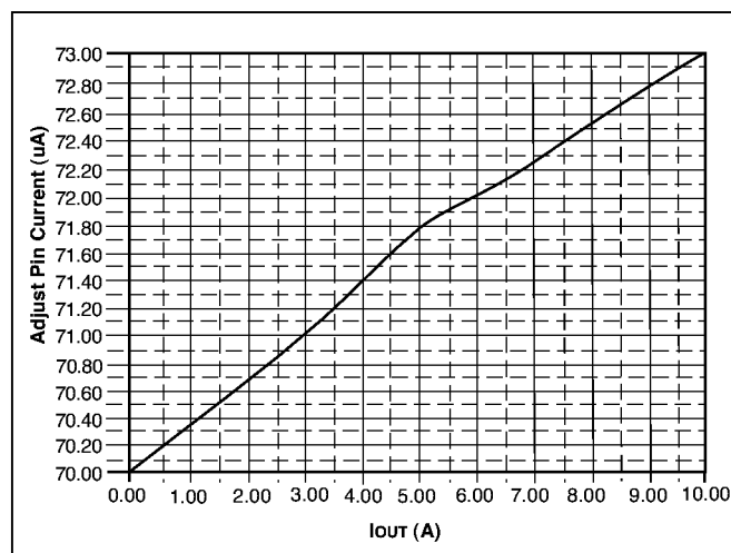
Adjust Pin Current vs I_{\text{OUT}}
