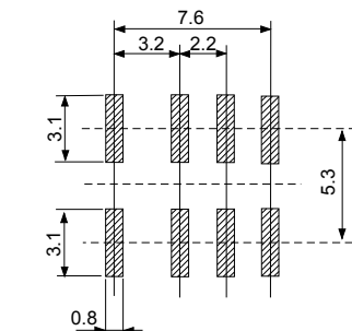
Recommended mounting pad (Tolerance: \pm 0.1\text{mm} )
