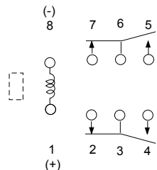
Terminal designations (Top view de-energized position)
