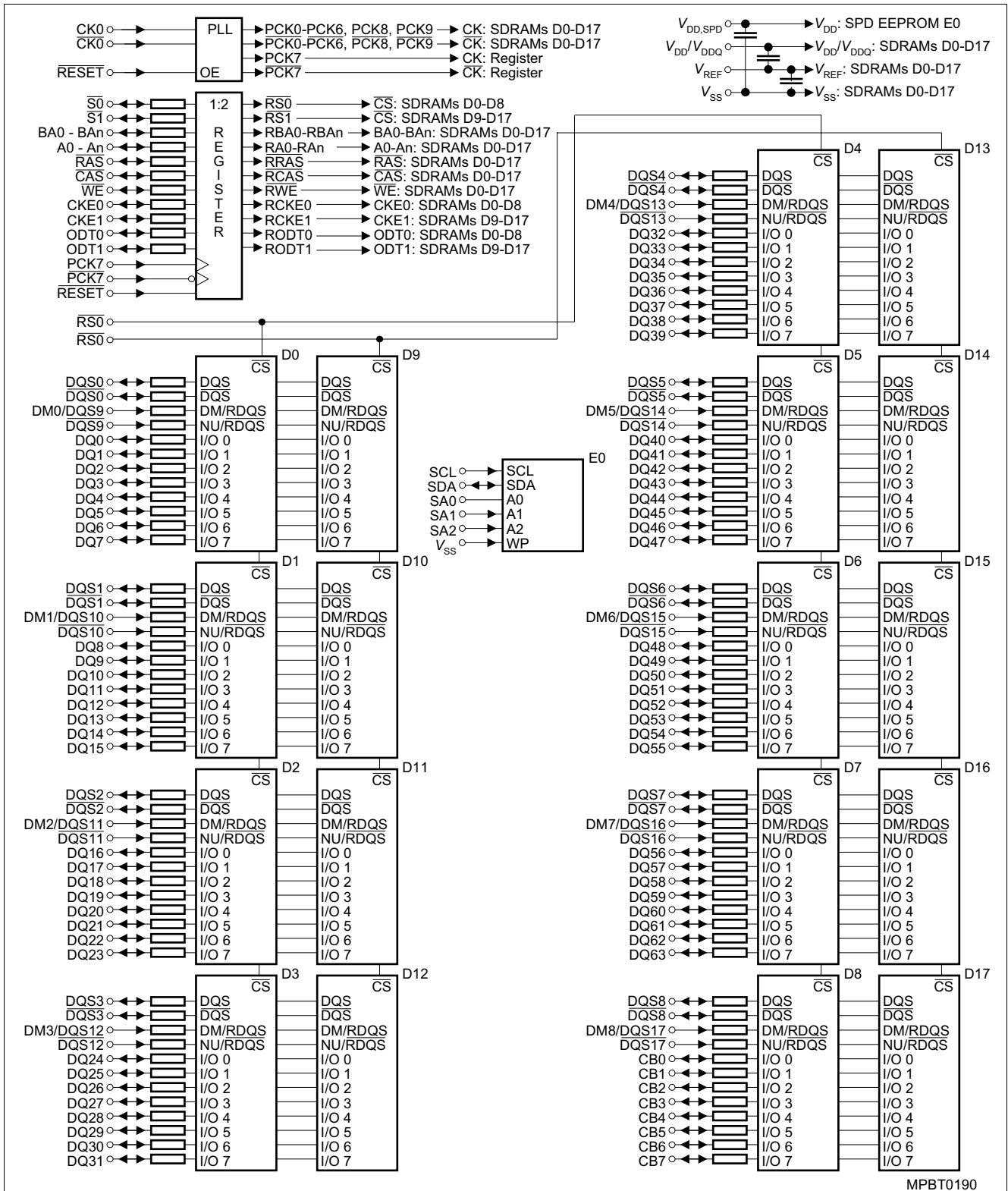
Figure 3 Block Diagram Raw Card G RDIMM (x72, 2Ranks, x8)
