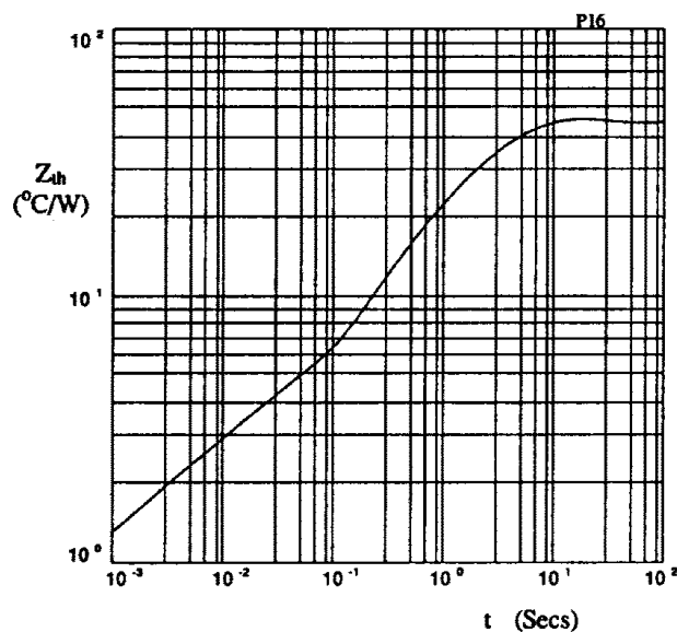
Fig 5. Transient thermal impedance characteristic.
