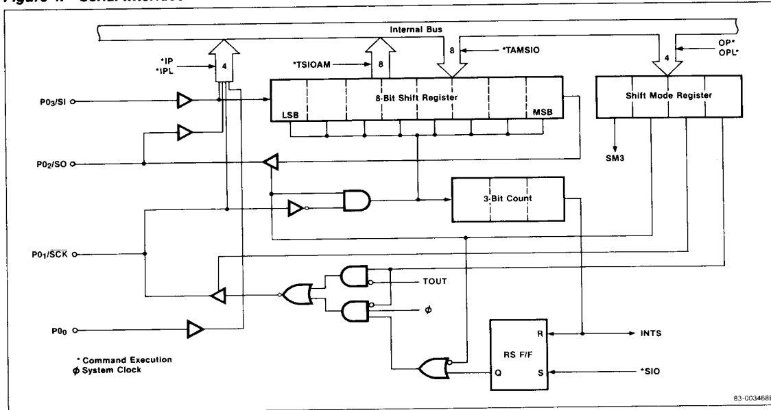
Figure 4. Serial Interface
