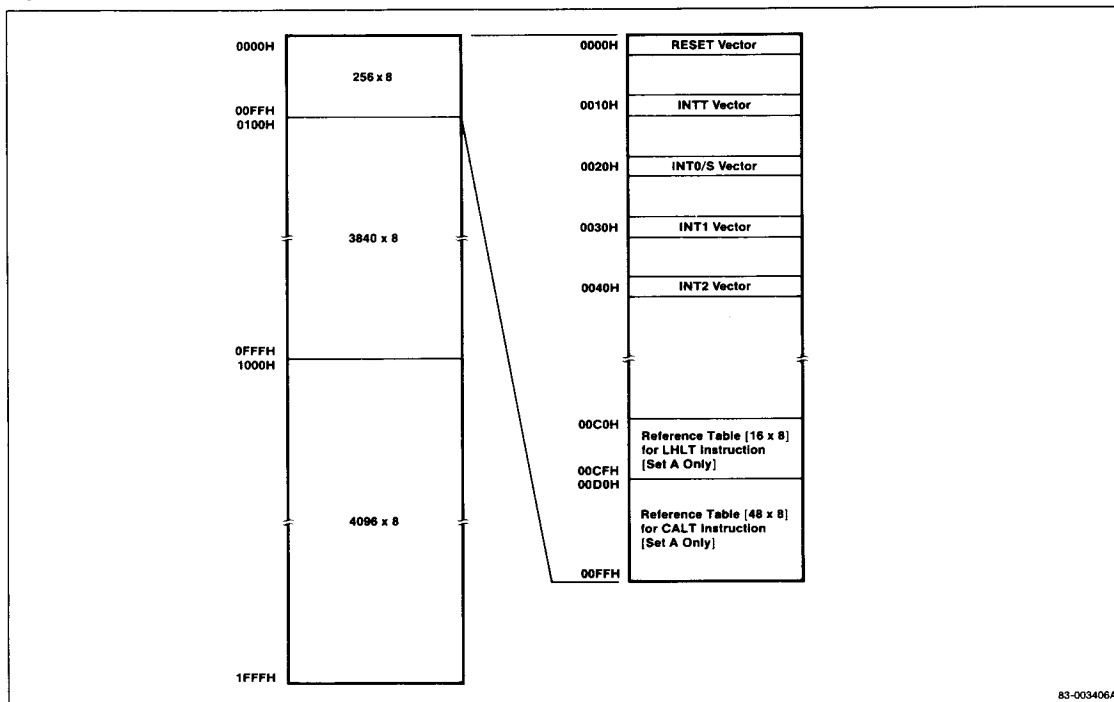
Figure 2. Program Memory Map
