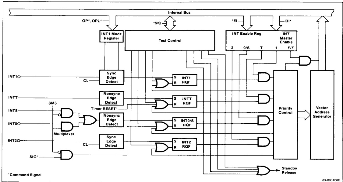
Figure 5. Interrupt Control
