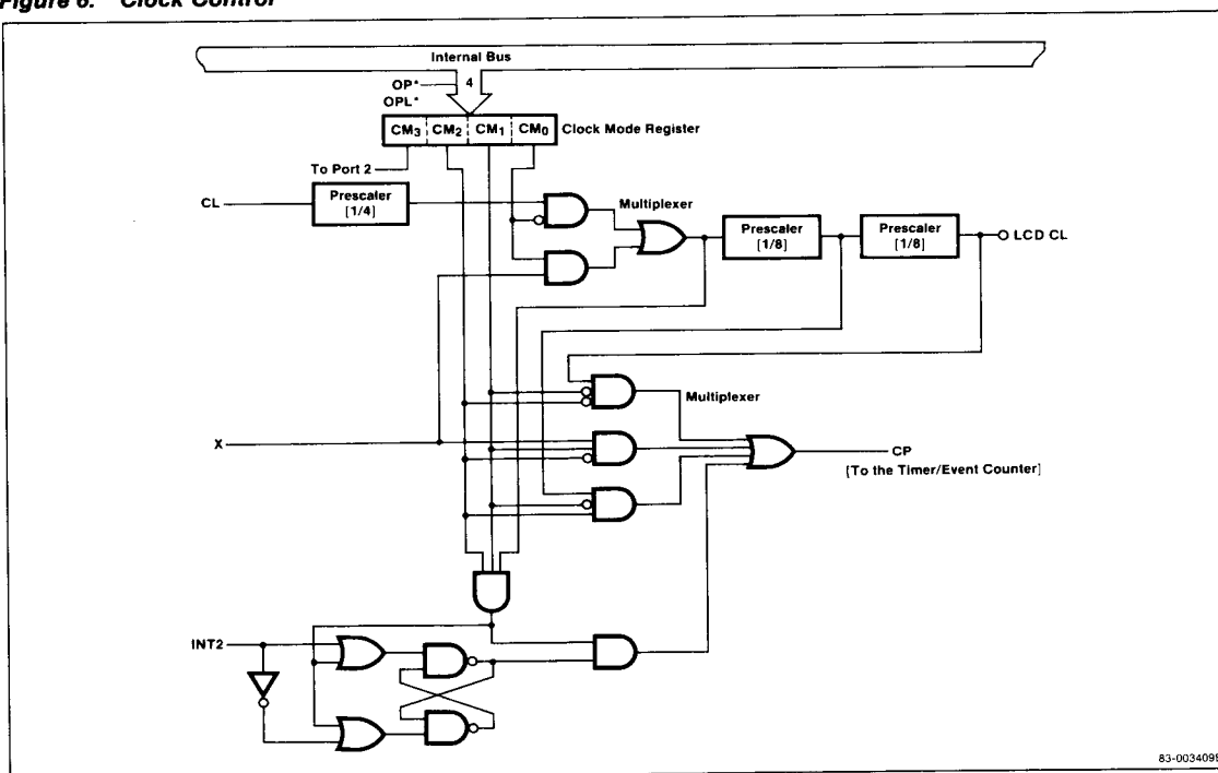
Figure 6. Clock Control
