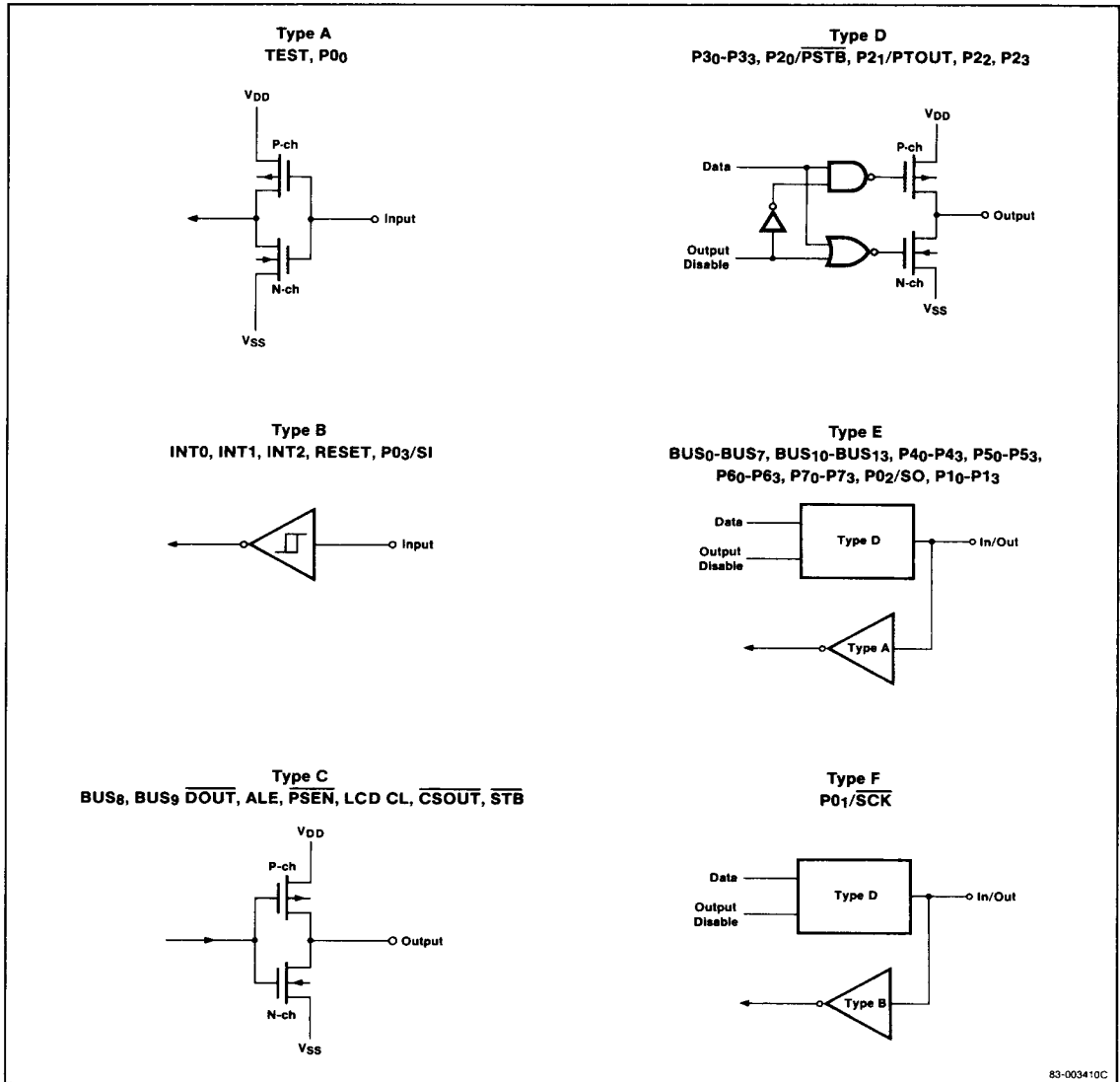
Figure 7. Interface at Input/Output Ports
