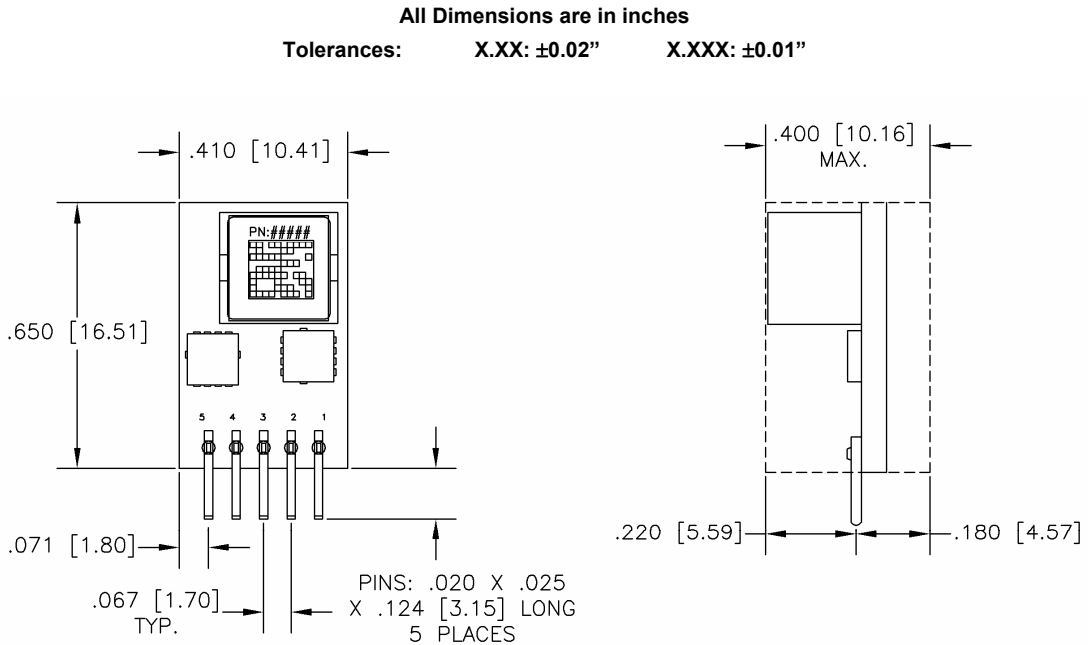
Figure 17. Mechanical Drawing
