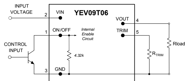
Figure 15. Circuit Configuration For ON/OFF Function
