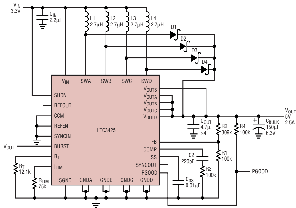
Figure 7. Application Circuit for V_{OUT} > 4.3V with Inrush Limiting and Output Disconnect
