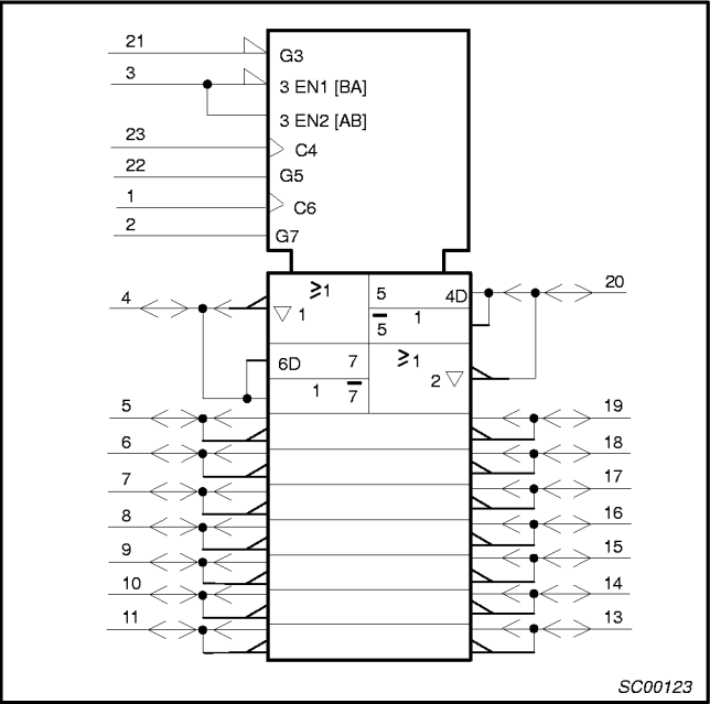
IEC/IEEE SYMBOL – 74ALS648/648-1
