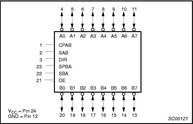
IEC/IEEE SYMBOL – 74ALS648/648-1
