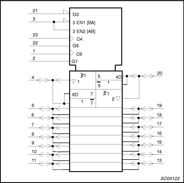
IEC/IEEE SYMBOL – 74ALS646/646-1
