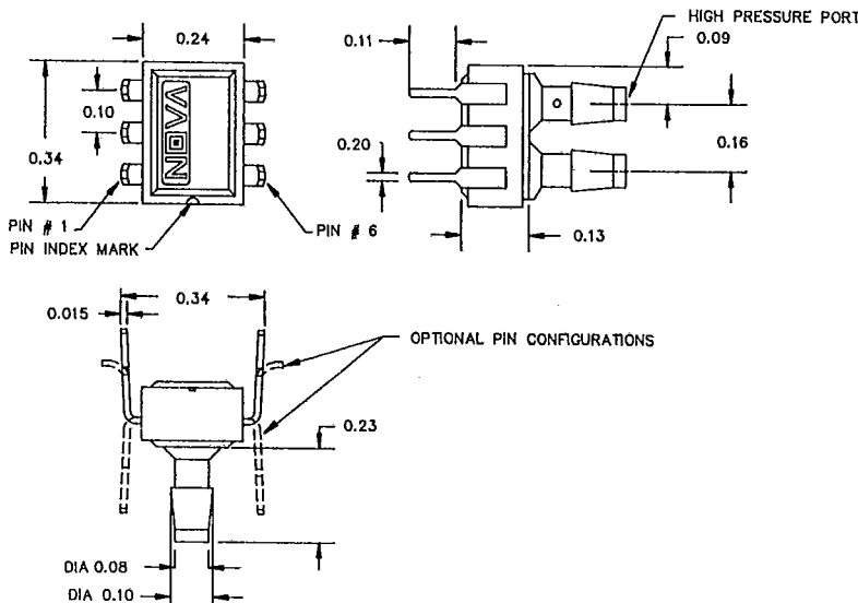
PACKAGE OUTLINE DIMENSIONS
