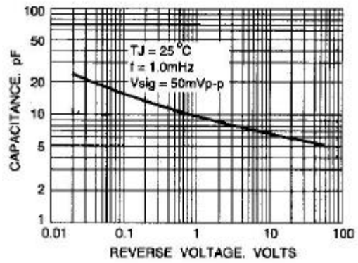
Fig. 6-TYPICAL JUNCTION CAPACITANCE
