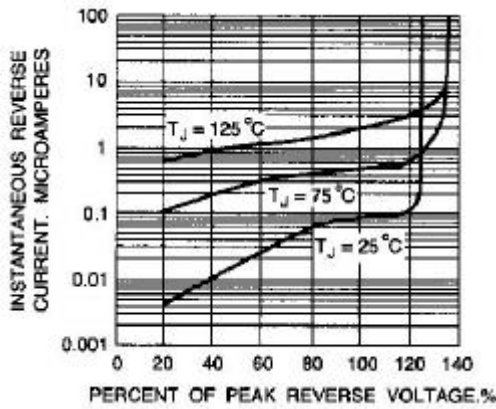
Fig. 3-TYPICAL REVERSE CHARACTERISTICS
