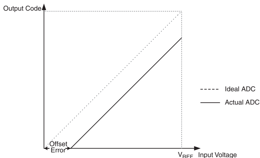
Figure 21-10. Offset Error
