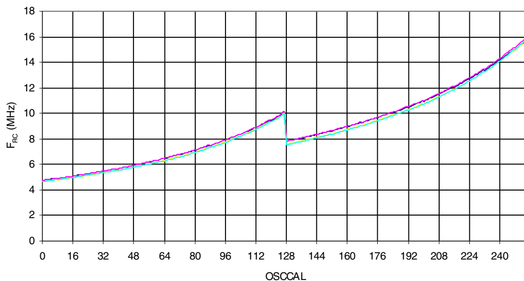
Figure 27-38. Calibrated 8 MHz RC Oscillator Frequency vs. Oscal Value
