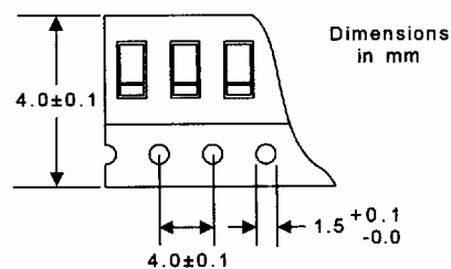
Tape Dimensions and Orientation For Surface Mount MELF Package
