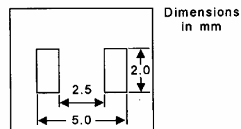
Mounting Pad Geometry For Surface Mount MELF Package
