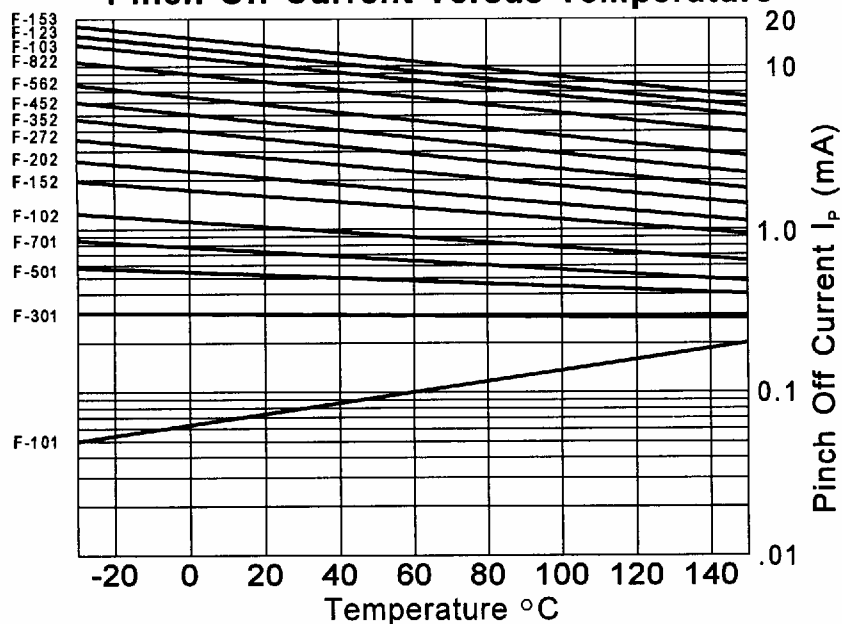
Pinch Off Current Versus Temperature
