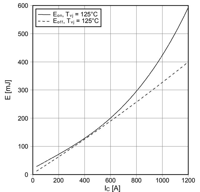
Schaltverluste IGBT-Wechselr. (typisch) switching losses IGBT-inverter (typical) E_{on} = f(I_c), E_{off} = f(I_c) V_{GE} = \pm 15\text{ V}, R_{Gon} = 2.4\ \Omega, R_{Goff} = 2.4\ \Omega, V_{CE} = 900\text{ V}
