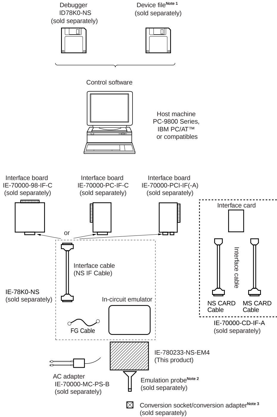
Figure 1-1. System Configuration
