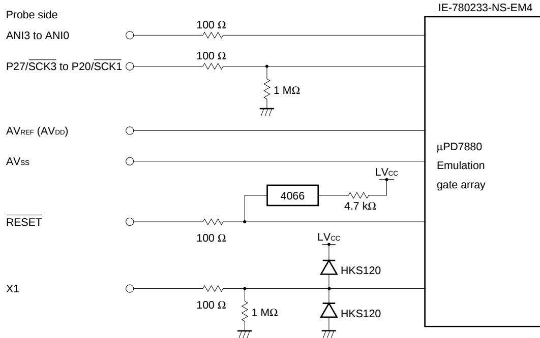
Figure 4-1. Equivalent Circuit of Emulation Circuit 1
