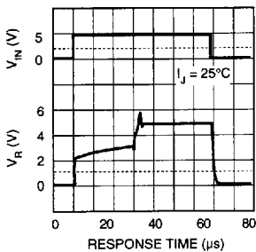
LM4040-2.5 R_S = 30\text{k}
