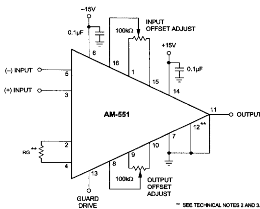
Figure 2. Typical Connections
