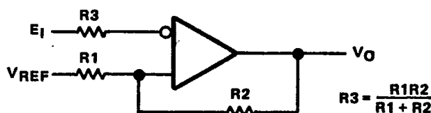
Figure 2-38. Comparator with Hysteresis
