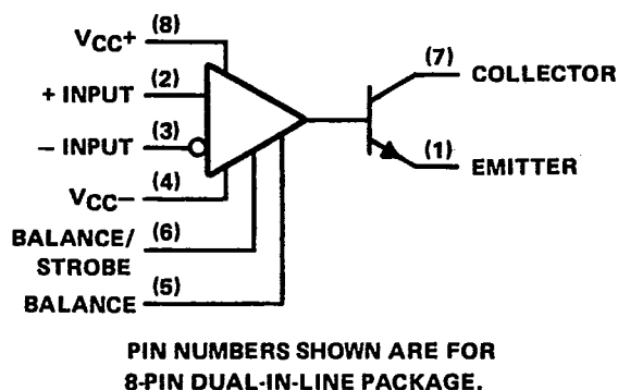
Figure 2-37. TLC311 or LM311 Comparator
