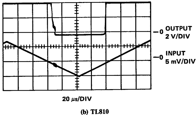
Figure 2-40. Response of a TL710 and a TL810 to a Ramp Input
