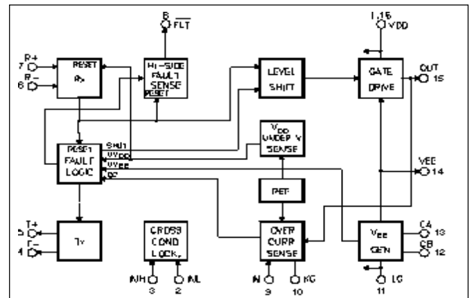
Block diagram IXBD 4411
