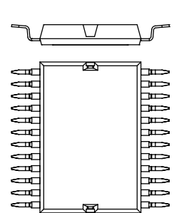
GMM 3x xxx - SMD SURFACE MOUNT DEVICE
