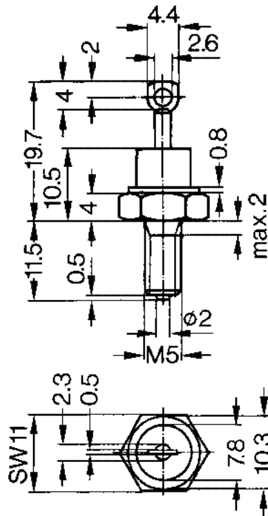
X204 DO-203 AA [M] (DO-4)
