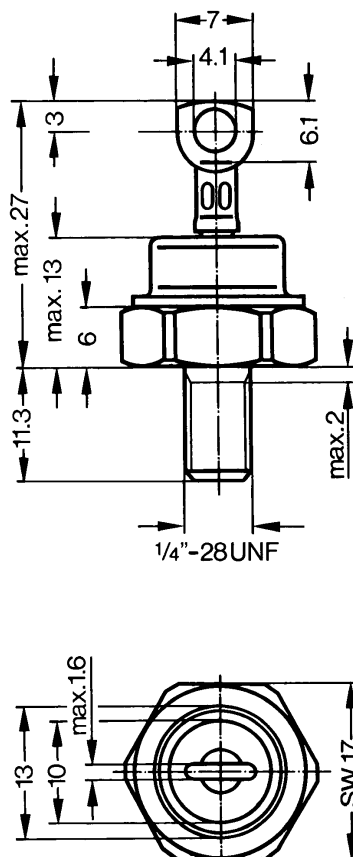
X207 DO-203 AB (DO-5)
