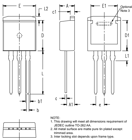
X008 TO-262 I 2 PAK
