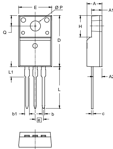
X007a TO-220 ABFP
