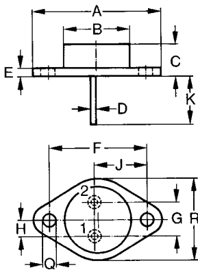
X203 TO-204 AE
