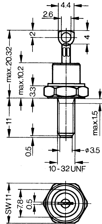
X205 DO-203 AA [UNF] (DO-4)
