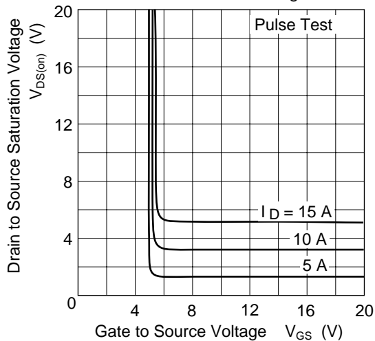
www.DataSheet4U.com Drain to Source Saturation Voltage vs. Gate to Source Voltage
