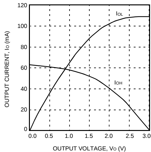
Figure 30. Fast ( T_j = 125^\circ\text{C} , V_{DD} = 3.0\text{ V} )
