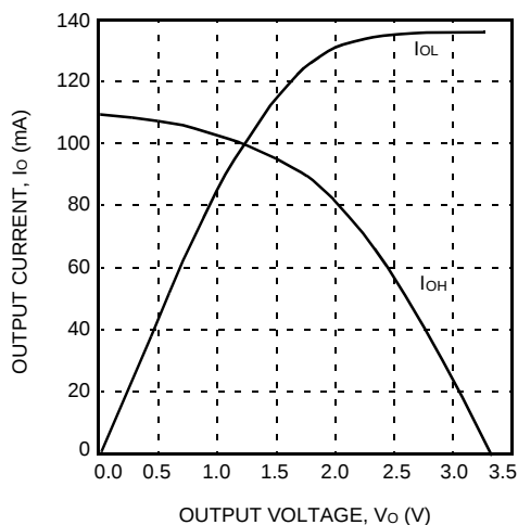
Figure 27. Fast ( T_j = 25^\circ\text{C} , V_{DD} = 3.3\text{ V} )
