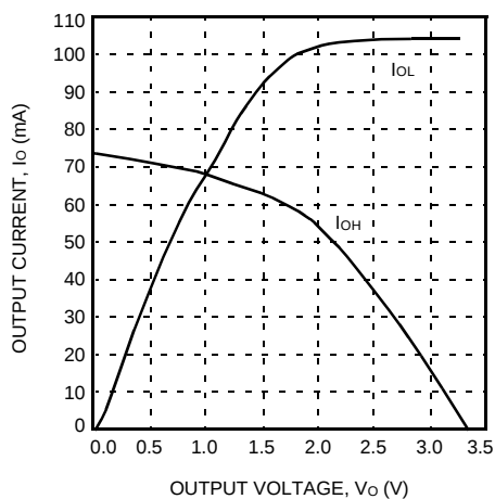
Figure 25. Sinklim ( T_j = 25^\circ\text{C} , V_{DD} = 3.3\text{ V} )
