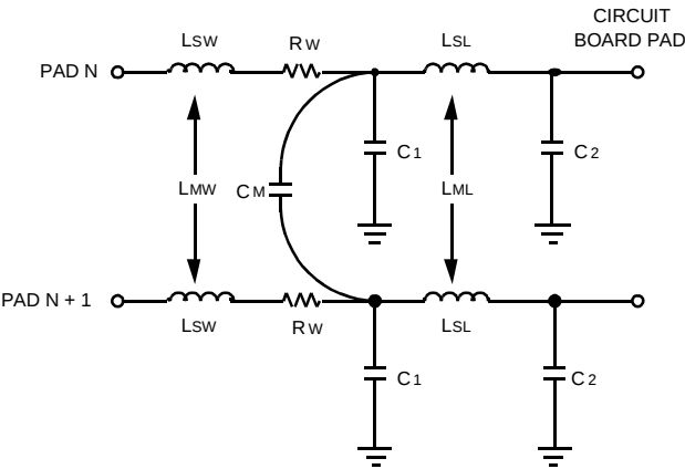
Figure 34. Package Parasitics
