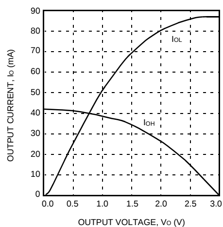
Figure 28. Sinklim ( T_j = 125^\circ\text{C} , V_{DD} = 3.0\text{ V} )
