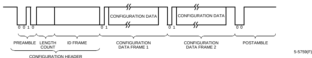
Figure 11. Serial Configuration Data Format—Autoincrement Mode
