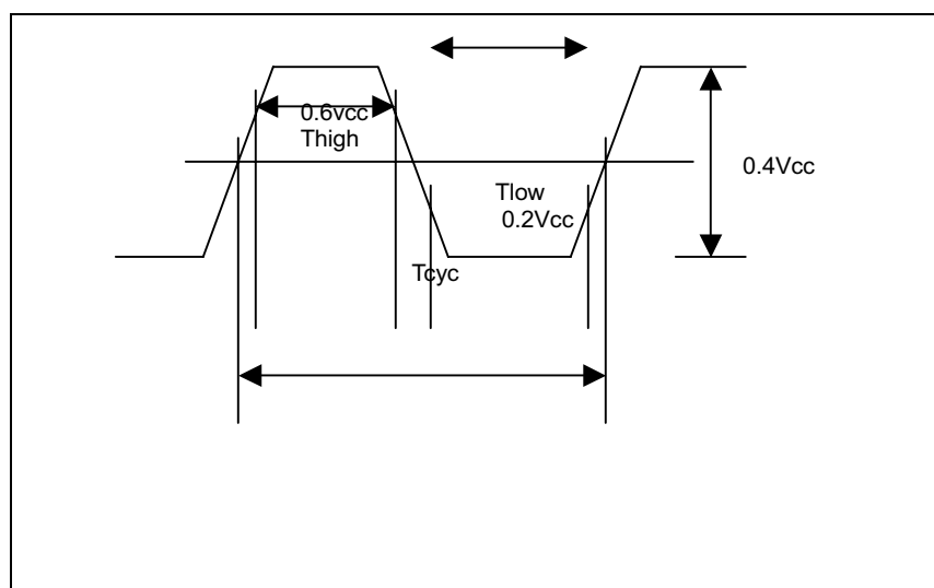
Figure 13 CARDBUS Clock Waveform
