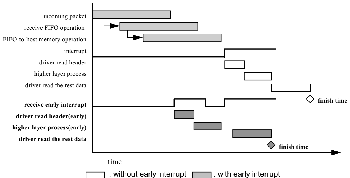
Fig.9 Receive data flow (without early interrupt and with early interrupt)
