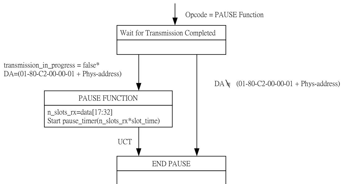
Fig.12 PAUSE operation receive state diagram
