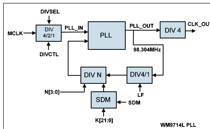
Figure 3 PLL Architecture
