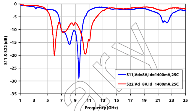
XP1050-QJ: S11 & S22 (Wideband) Vd=8V, Idtot=1400mA
