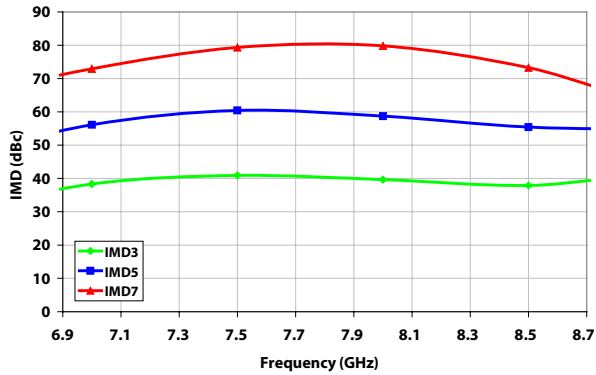
XP1050-QJ: IMD3,IMD5,IMD7 Pout/tone=25.5dBm,Vd=8V,Id=1200mA
