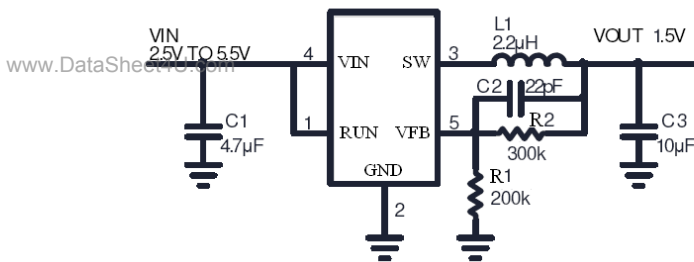
Figure 1. Basic Application Circuit with AP2406 adjustable version
