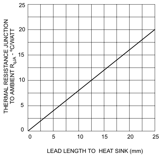
Typical Thermal Resistance (Using Standard Mounting Method "B")
