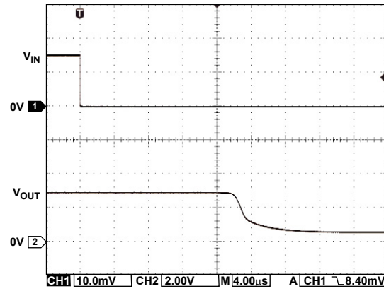
Figure 43. Positive Overload Recovery (Gain = 1280)
