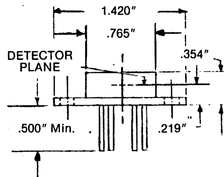
TO-3 PLATE CELL
