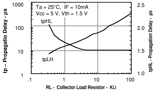
Figure 17. Propagation delay versus collector load resistor
