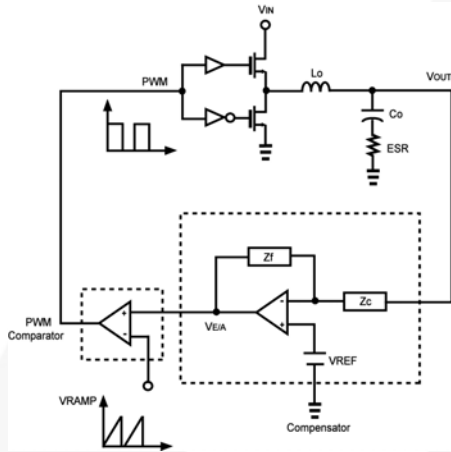
Figure 24. Closed Loop
