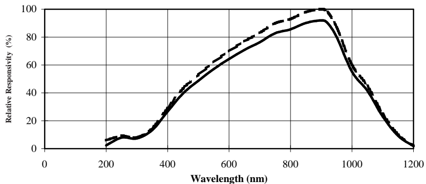
Spectral Response
