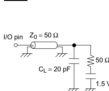
Fig.1: AC test load
