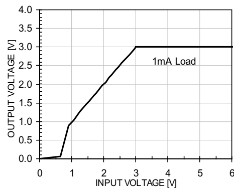
Figure 6. Line Regulation ( I_{LOAD}=1\text{mA} )
