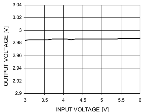
Figure 5. Line Regulation ( I_{LOAD}=5\text{mA} )
