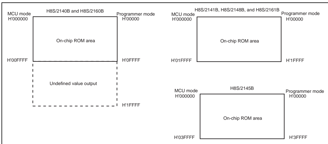
Figure 23.13 Memory Map in Programmer Mode
