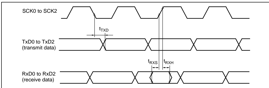
Figure 28.24 SCI Input/Output Timing (Synchronous Mode)
