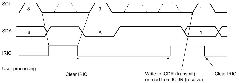
Figure 16.27 IRIC Setting Timing and SCL Control (2)
