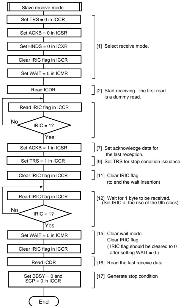
Figure 16.15 Sample Flowchart for Operations in Master Receive Mode (receiving a single byte) (WAIT = 1)
