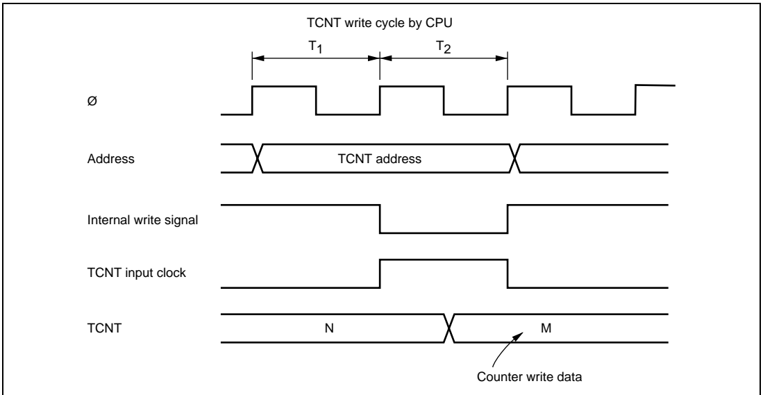
Figure 12.15 Conflict between TCNT Write and Increment
