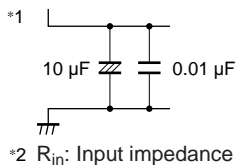
Figure 21.8 Example of Analog Input Protection Circuit
