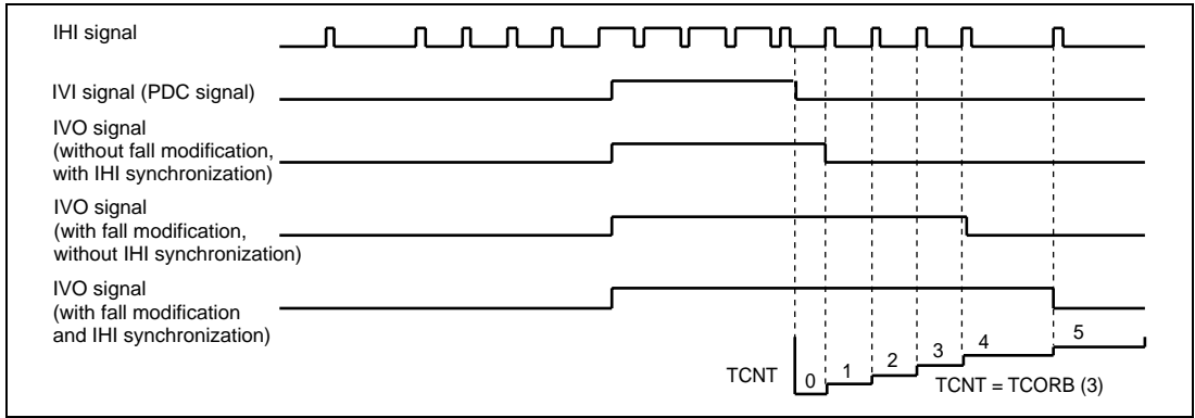
Figure 13.7 Fall Modification and IHI Synchronization Timing Chart
