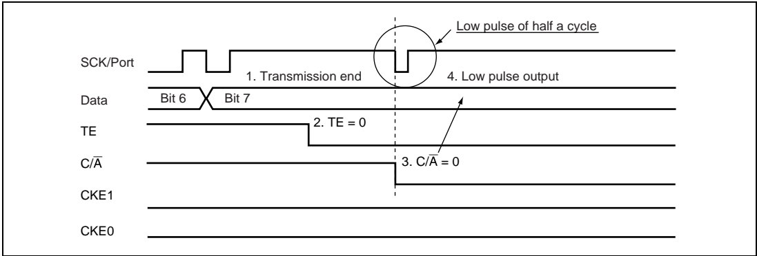
Figure 15.28 Switching from SCK Pins to Port Pins
