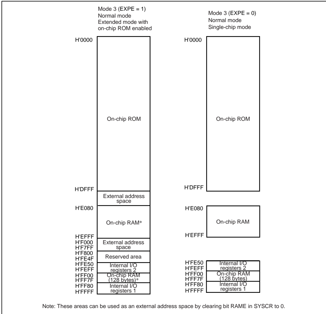
Figure 3.8 Address Map for H8S/2148B (2)
