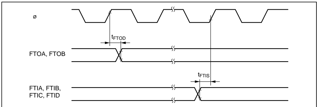
Figure 28.17 FRT Input/Output Timing
