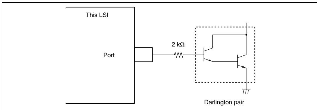
Figure 28.1 Darlington Pair Drive Circuit (Example)
