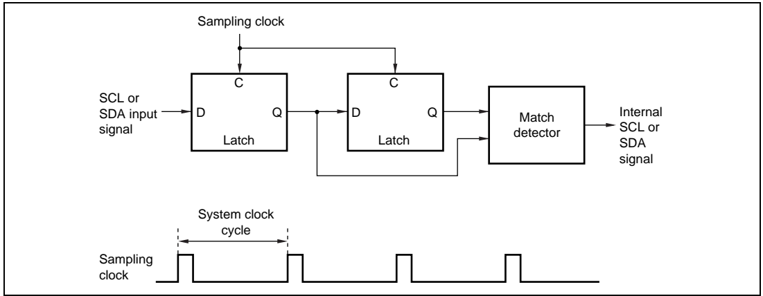
Figure 16.29 Block Diagram of Noise Canceler
