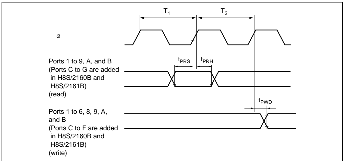
Figure 28.16 I/O Port Input/Output Timing
