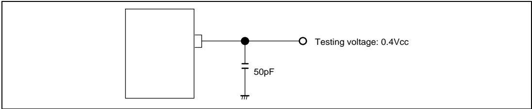
Figure 28.31 Tester Measurement Condition
