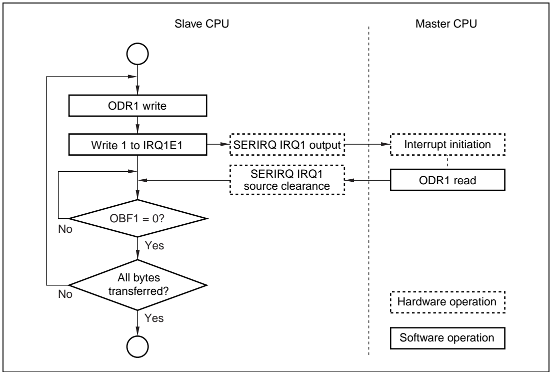
Figure 19.8 HIRQ Flowchart (Example of Channel 1)
