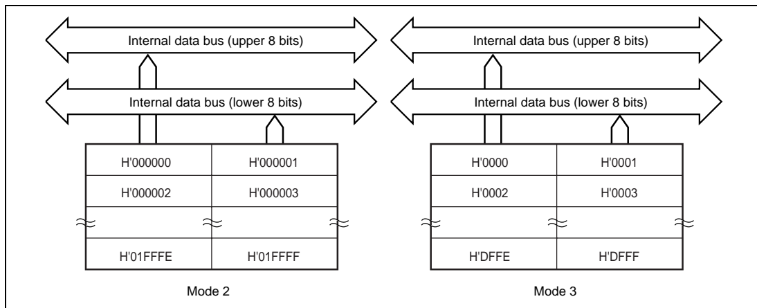
Figure 24.1 Block Diagram of 128-Kbyte Masked ROM (HD6432161BV)
