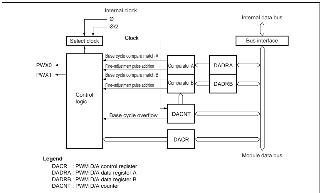
Figure 10.1 PWM (D/A) Block Diagram
