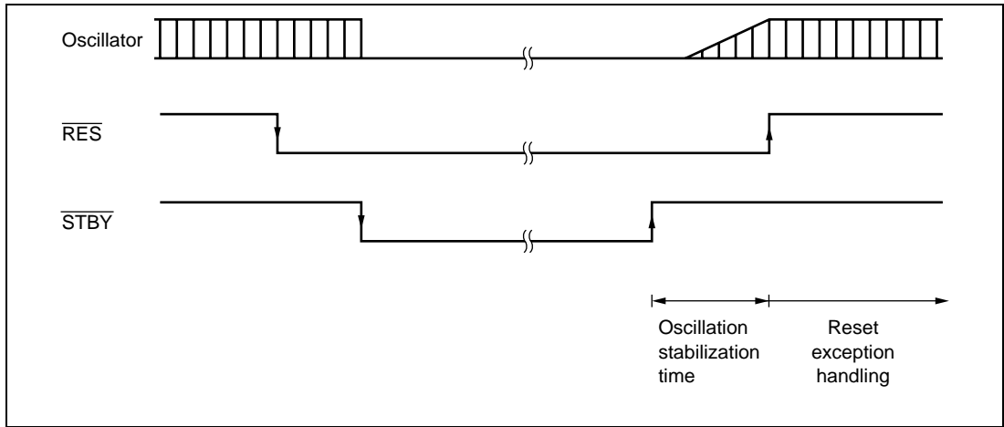
Figure 26.4 Hardware Standby Mode Timing
