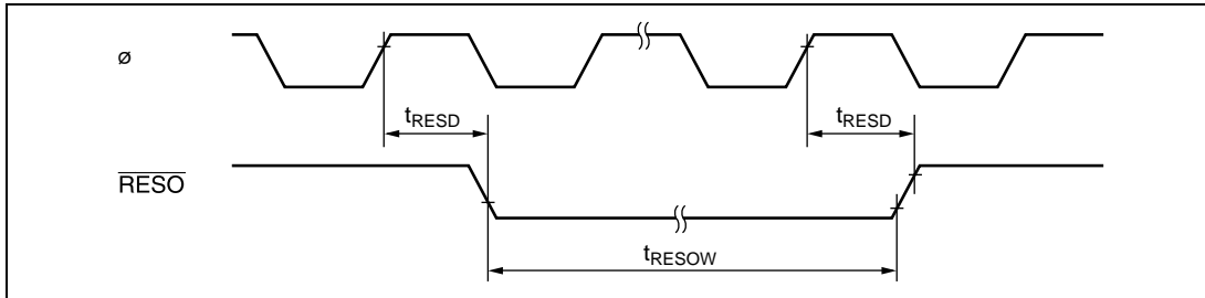
Figure 28.26 WDT Output Timing ( \overline{\text{RESO}} )
