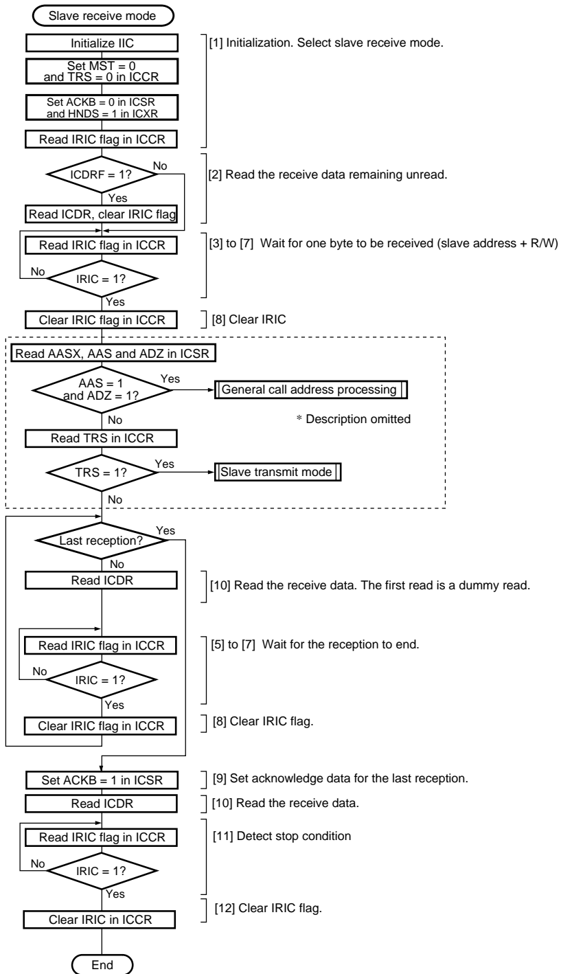
Figure 16.18 Sample Flowchart for Operations in Slave Receive Mode (HNDS = 1)
