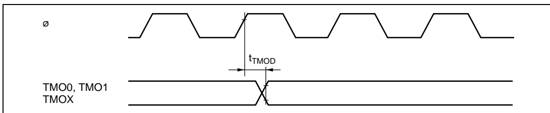
Figure 28.19 8-Bit Timer Output Timing
