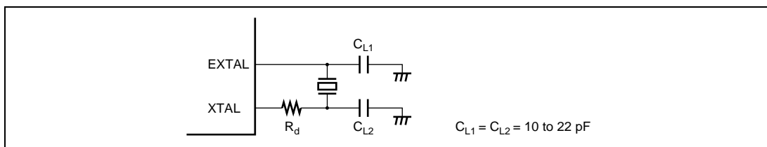
Figure 25.2 Typical Connection to Crystal Resonator
