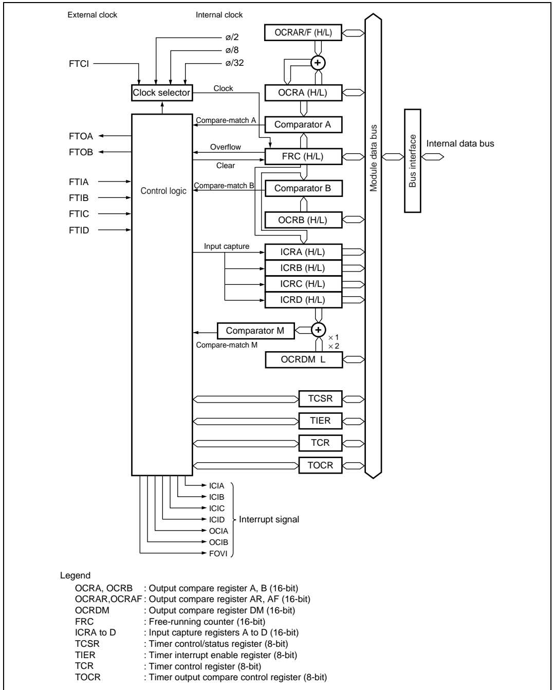
Figure 11.1 Block Diagram of 16-Bit Free-Running Timer
