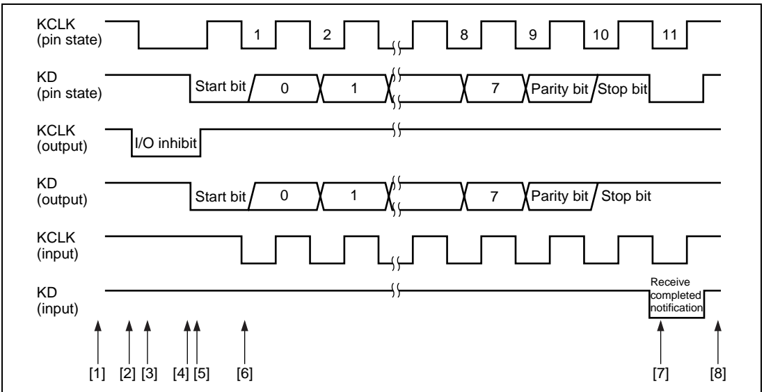
Figure 17.6 Transmit Timing
