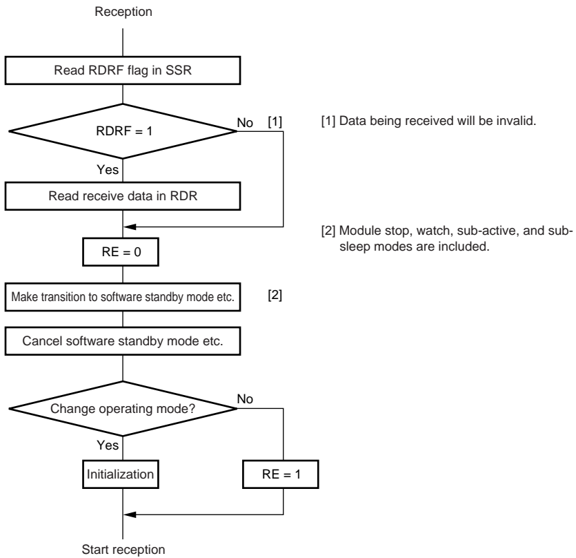
Figure 15.27 Sample Flowchart for Mode Transition during Reception
