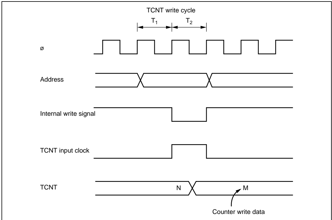
Figure 14.7 Conflict between TCNT Write and Increment
