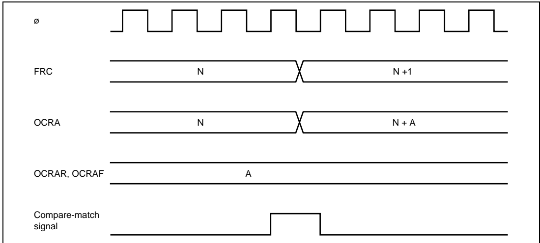
Figure 11.14 OCRA Automatic Addition Timing
