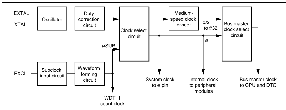
Figure 25.1 Block Diagram of Clock Pulse Generator
