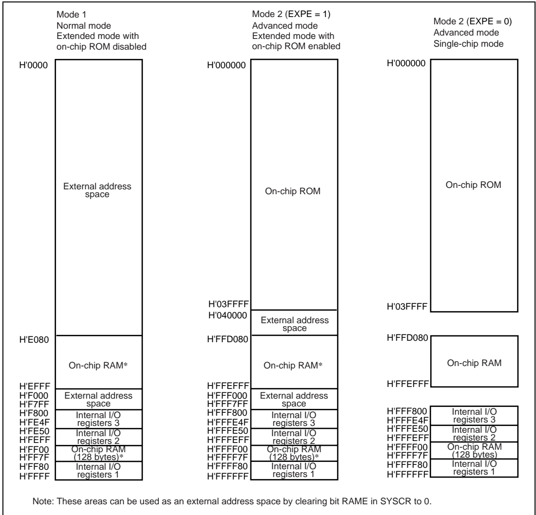
Figure 3.5 Address Map for H8S/2145BV (1)
