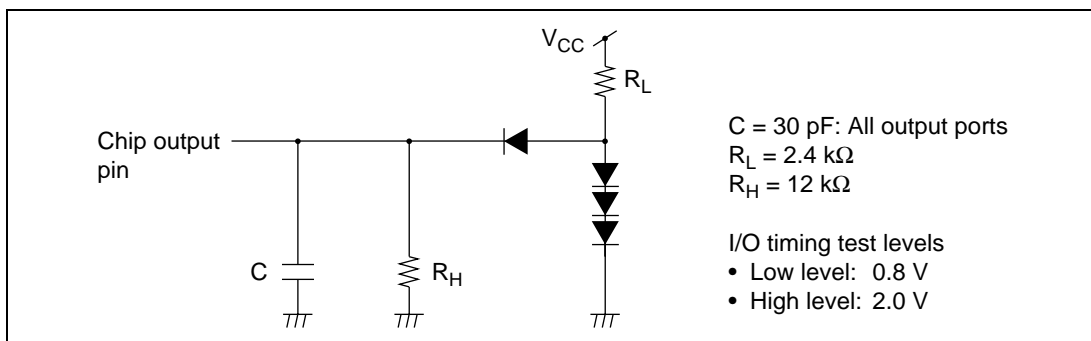
Figure 28.3 Output Load Circuit
