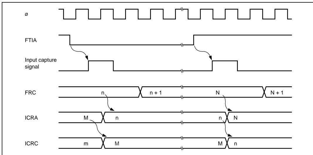
Figure 11.9 Buffered Input Capture Timing
