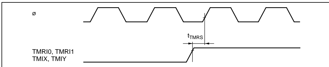
Figure 28.21 8-Bit Timer Reset Input Timing
