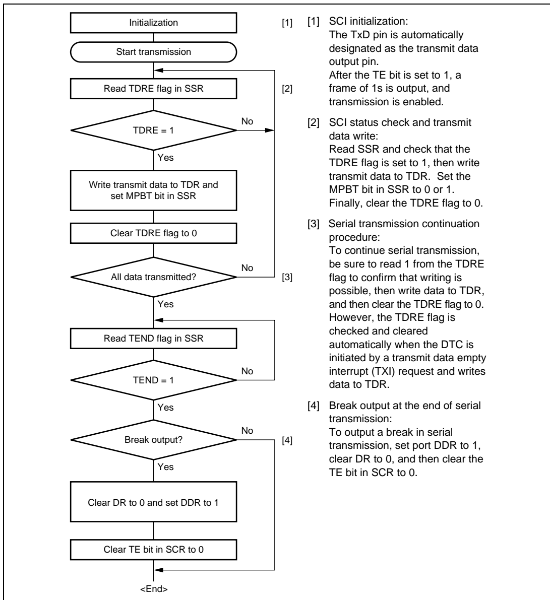
Figure 15.11 Sample Multiprocessor Serial Transmission Flowchart
