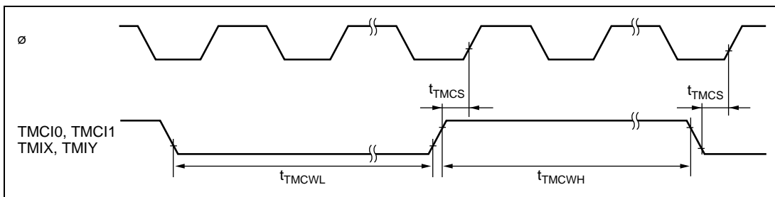
Figure 28.20 8-Bit Timer Clock Input Timing
