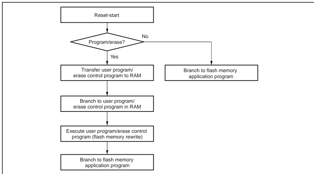
Figure 23.10 Programming/Erasing Flowchart Example in User Program Mode
