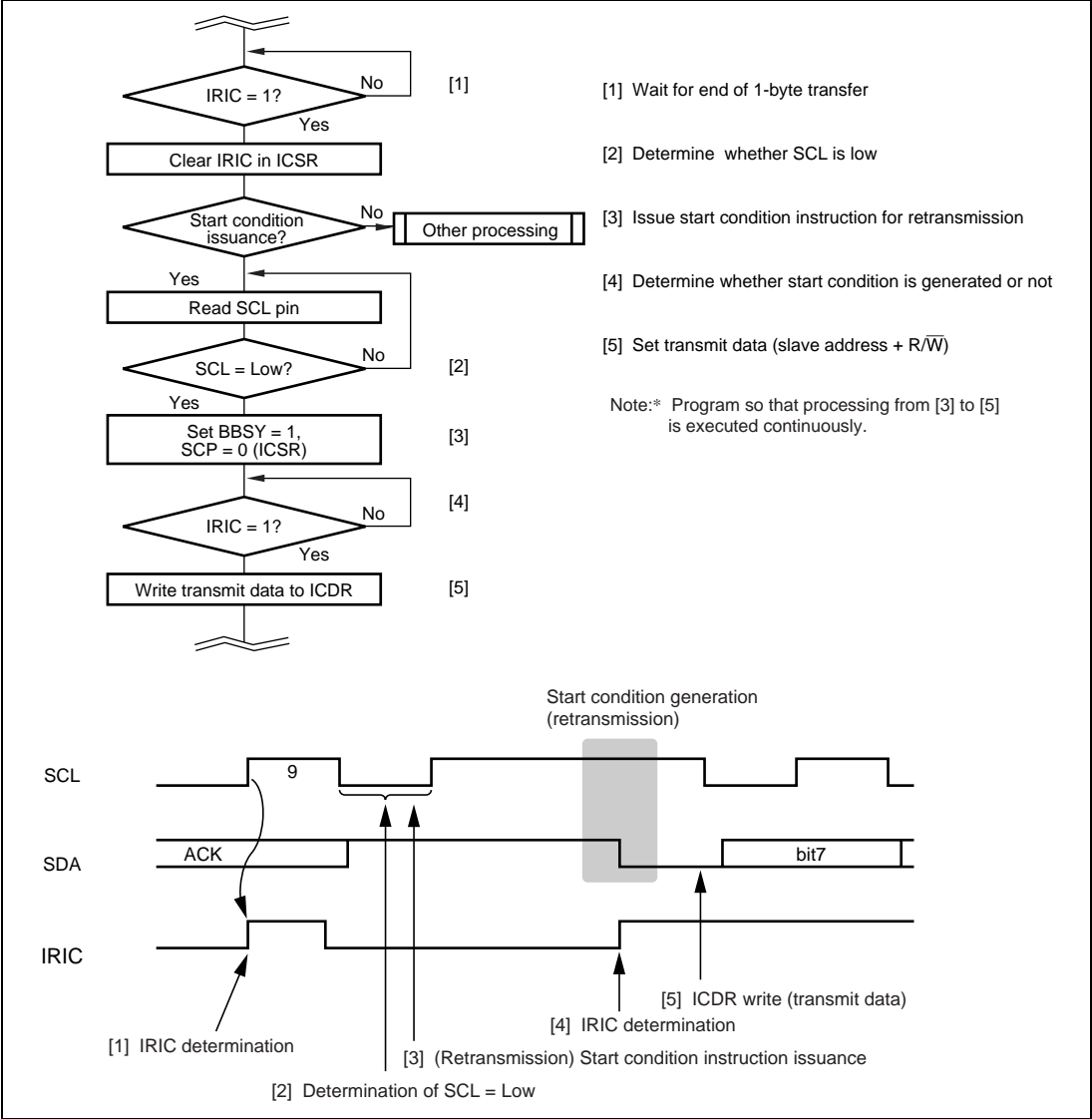
Figure 16.31 Flowchart for Start Condition Issuance Instruction for Retransmission and Timing
