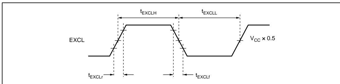
Figure 25.7 Subclock Input Timing
