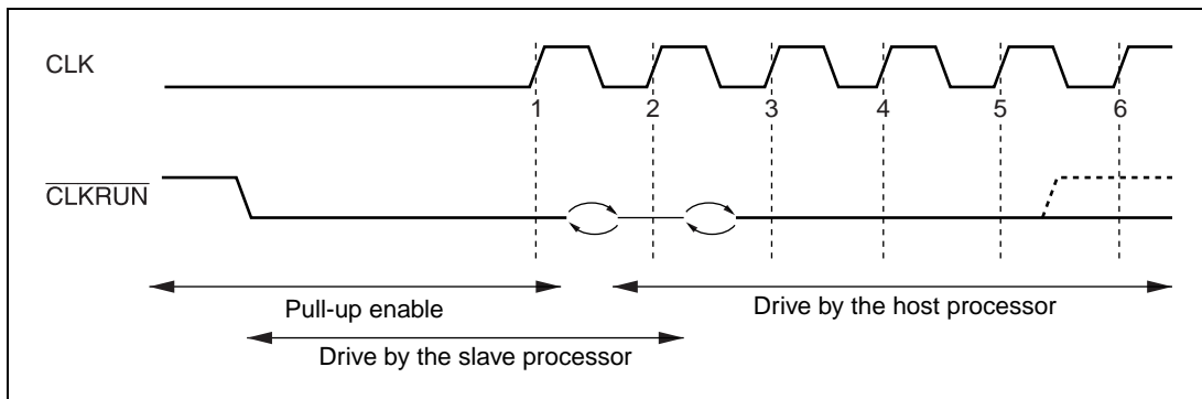
Figure 19.7 Clock Start Request Timing
