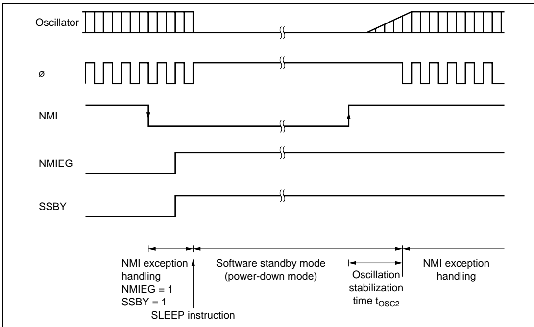
Figure 26.3 Application Example in Software Standby Mode
