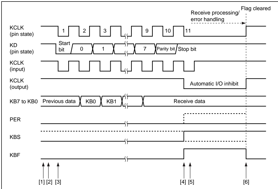
Figure 17.4 Receive Timing
