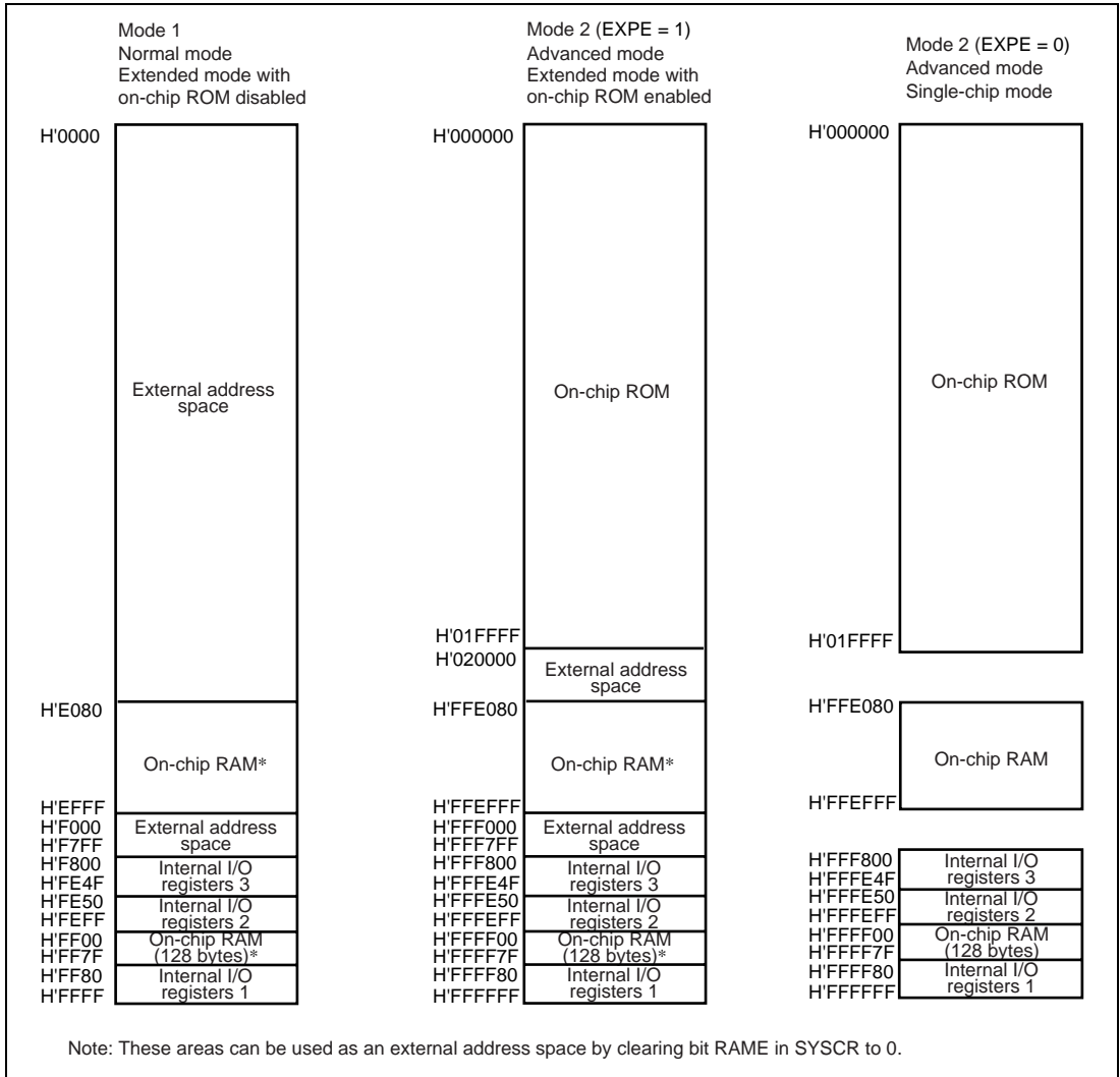
Figure 3.3 Address Map for H8S/2141B and H8S/2161B (1)
