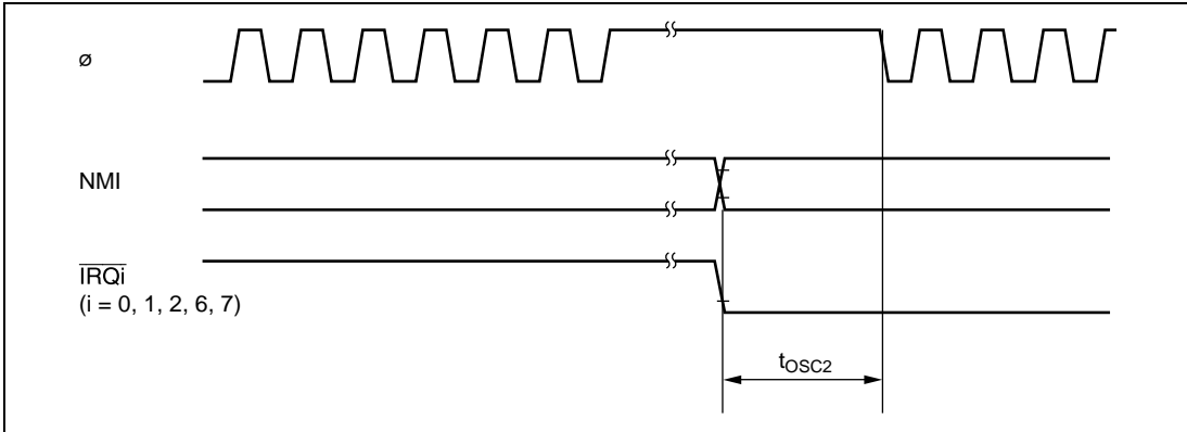
Figure 28.8 Oscillation Settling Timing (Exiting Software Standby Mode)
