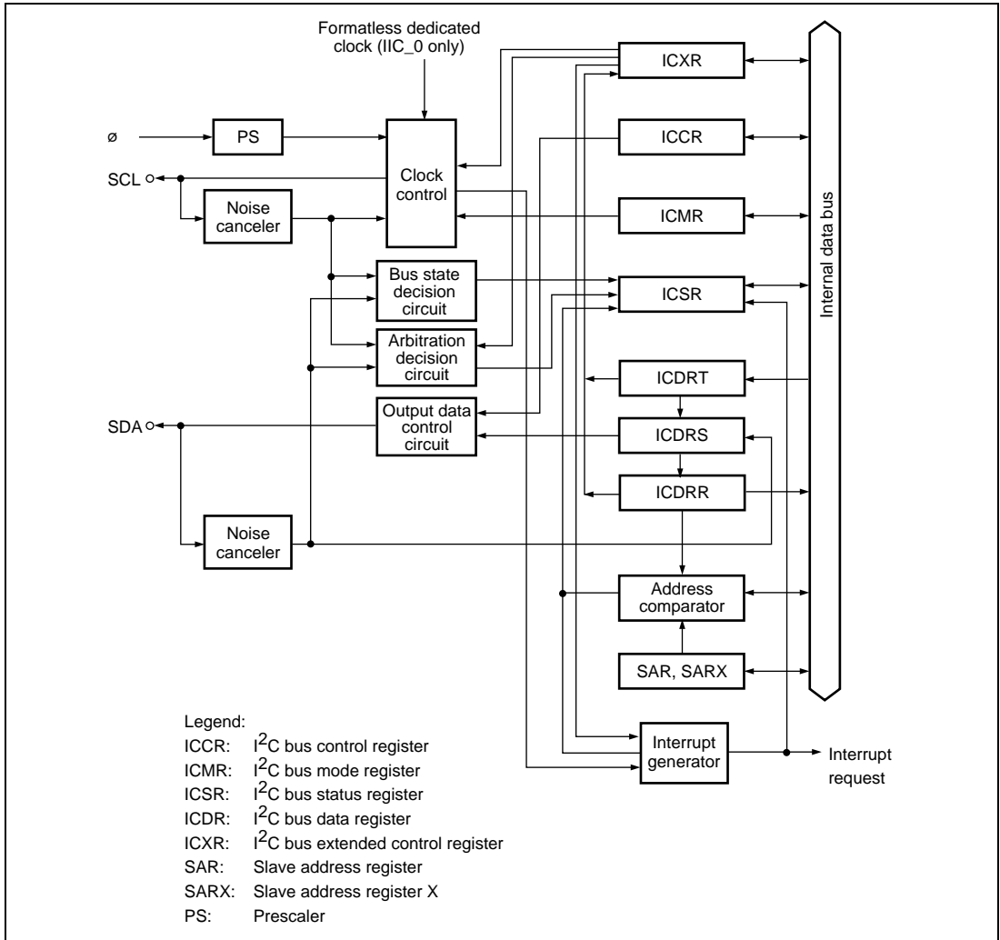
Figure 16.1 Block Diagram of I 2 C Bus Interface
