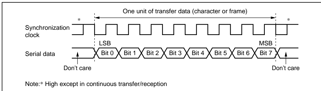
Figure 15.14 Data Format in Clocked Synchronous Communication (LSB-First)
