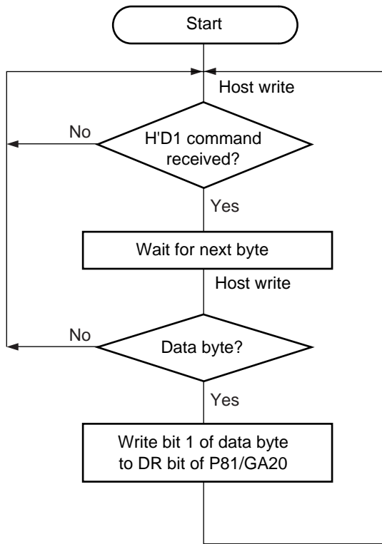
Figure 19.4 GA20 Output
