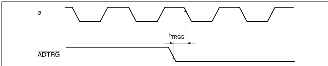
Figure 28.25 A/D Converter External Trigger Input Timing
