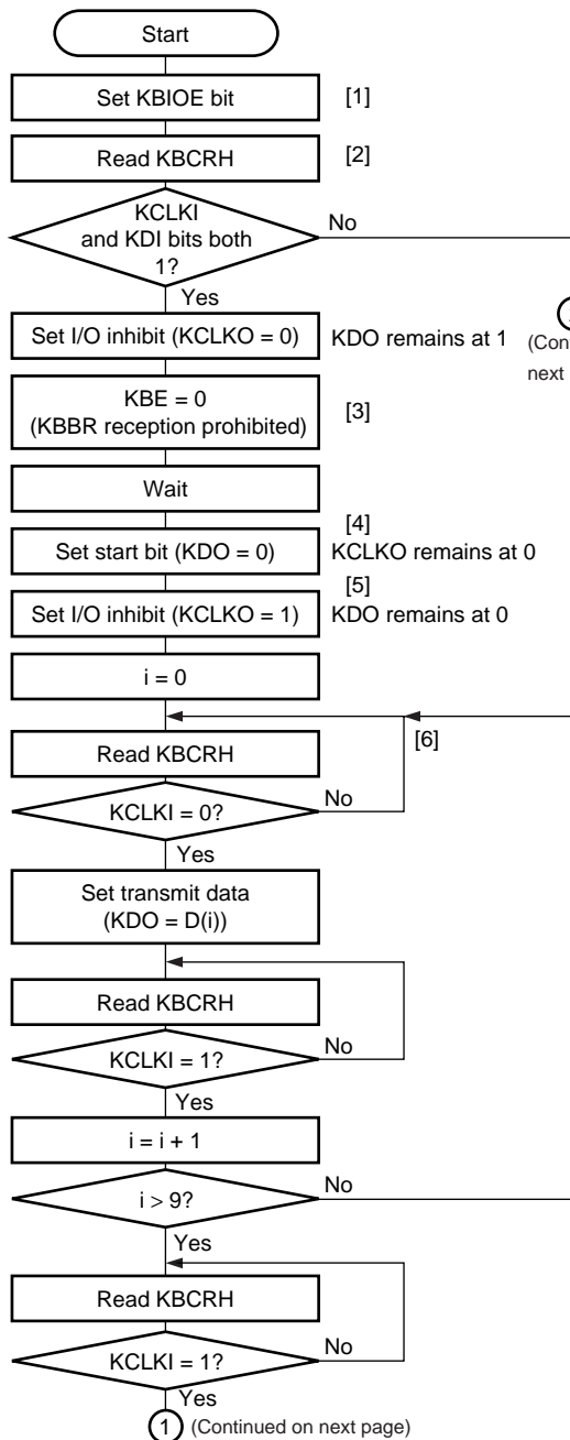
Figure 17.5 (1) Sample Transmit Processing Flowchart
