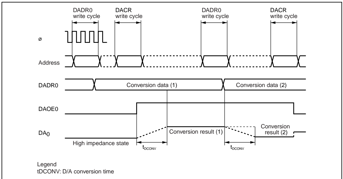
Figure 20.2 D/A Converter Operation Example
