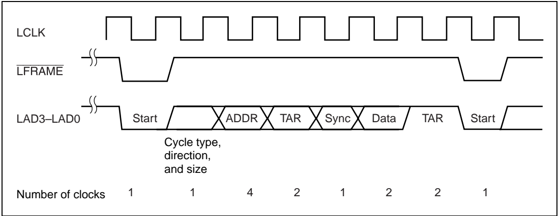
Figure 19.2 Typical \overline{\text{LFRAME}} Timing
