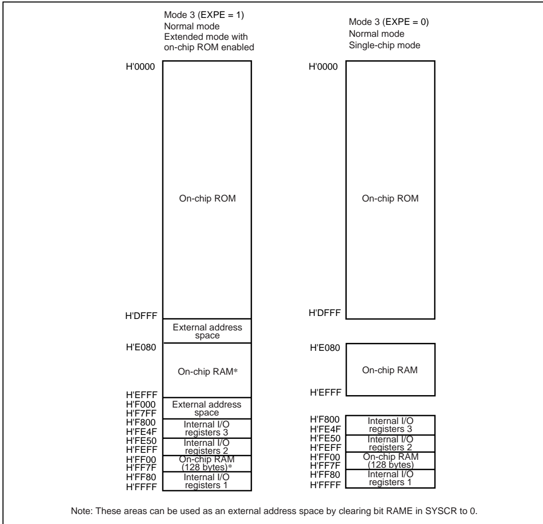
Figure 3.6 Address Map for H8S/2145BV (2)
