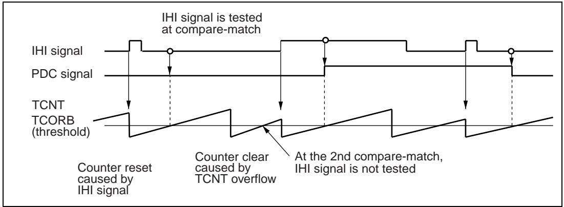
Figure 13.2 Timing Chart for PWM Decoding
