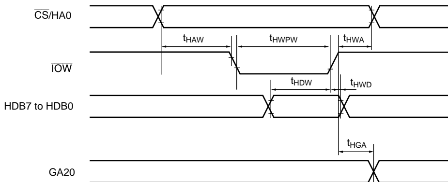
Figure 28.27 Host Interface (XBS) Timing
