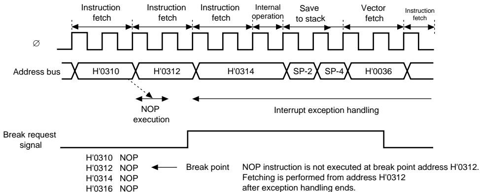
Figure 5.10 Address Break Timing Example
