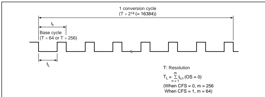
Figure 10.2 PWM D/A Operation
