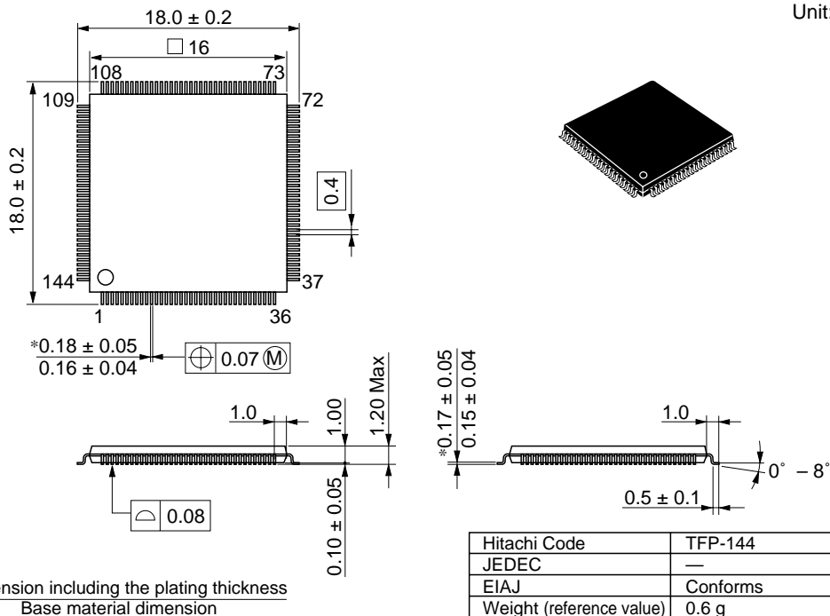
Figure C.3 Package Dimensions (TFP-144)
