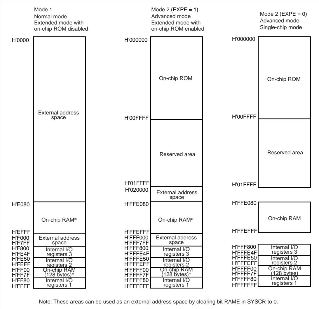
Figure 3.1 Address Map for H8S/2140B and H8S/2160B (1)
