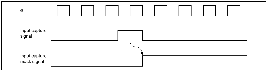
Figure 11.15 Timing of Input Capture Mask Signal Setting
