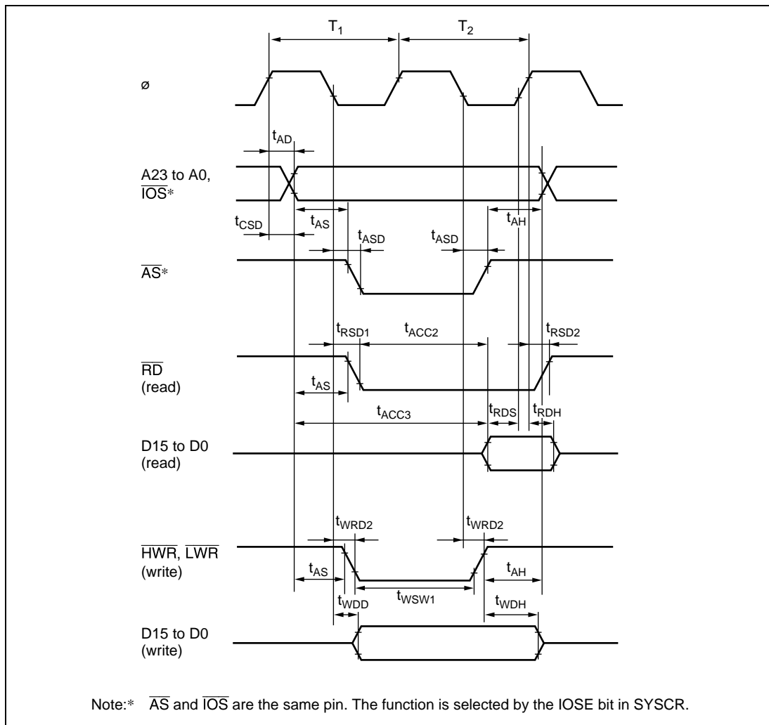
Figure 28.11 Basic Bus Timing (Two-State Access)
