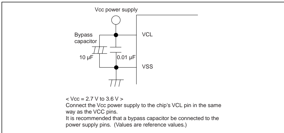
Figure 28.4 Connection of VCL Capacitor
