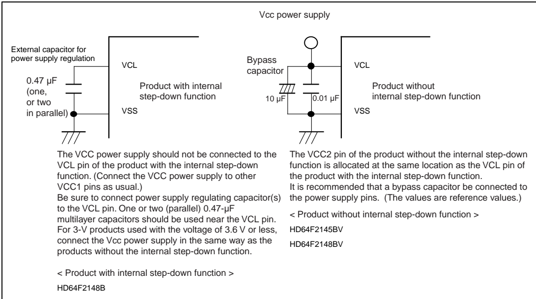
Figure 28.5 Connection of VCL Capacitor
