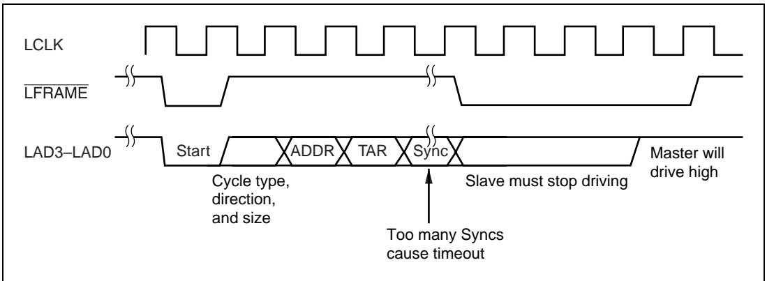
Figure 19.3 Abort Mechanism
