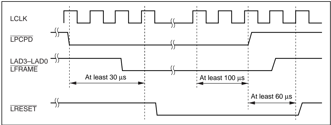
Figure 19.5 Power-Down State Termination Timing
