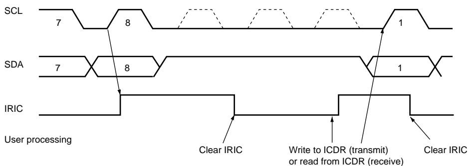
Figure 16.28 IRIC Setting Timing and SCL Control (3)
