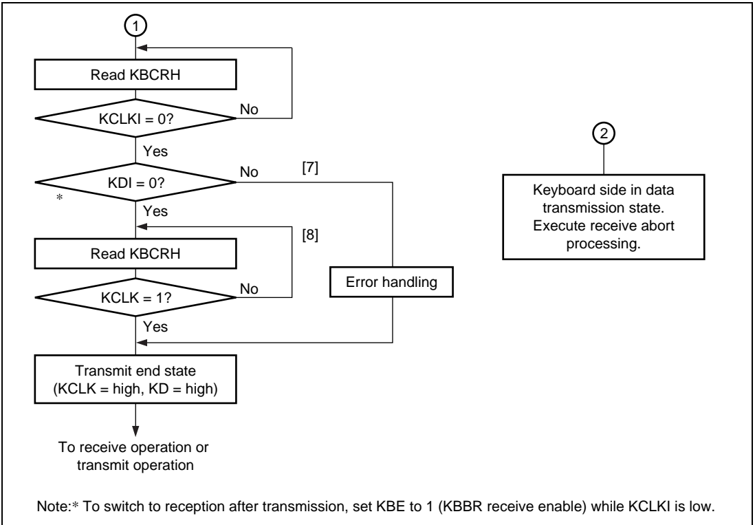
Figure 17.5 (2) Sample Transmit Processing Flowchart
