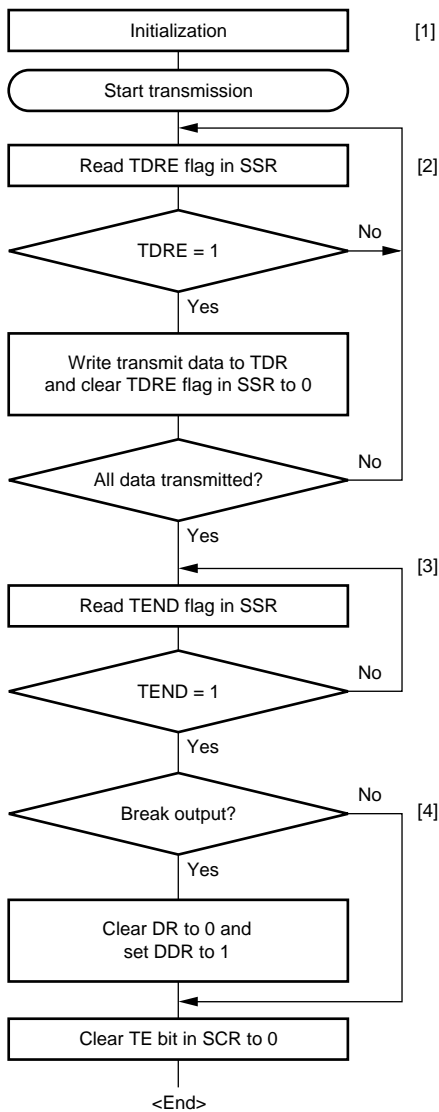
Figure 15.7 Sample Serial Transmission Flowchart
