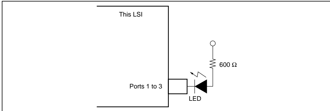
Figure 28.2 LED Drive Circuit (Example)
