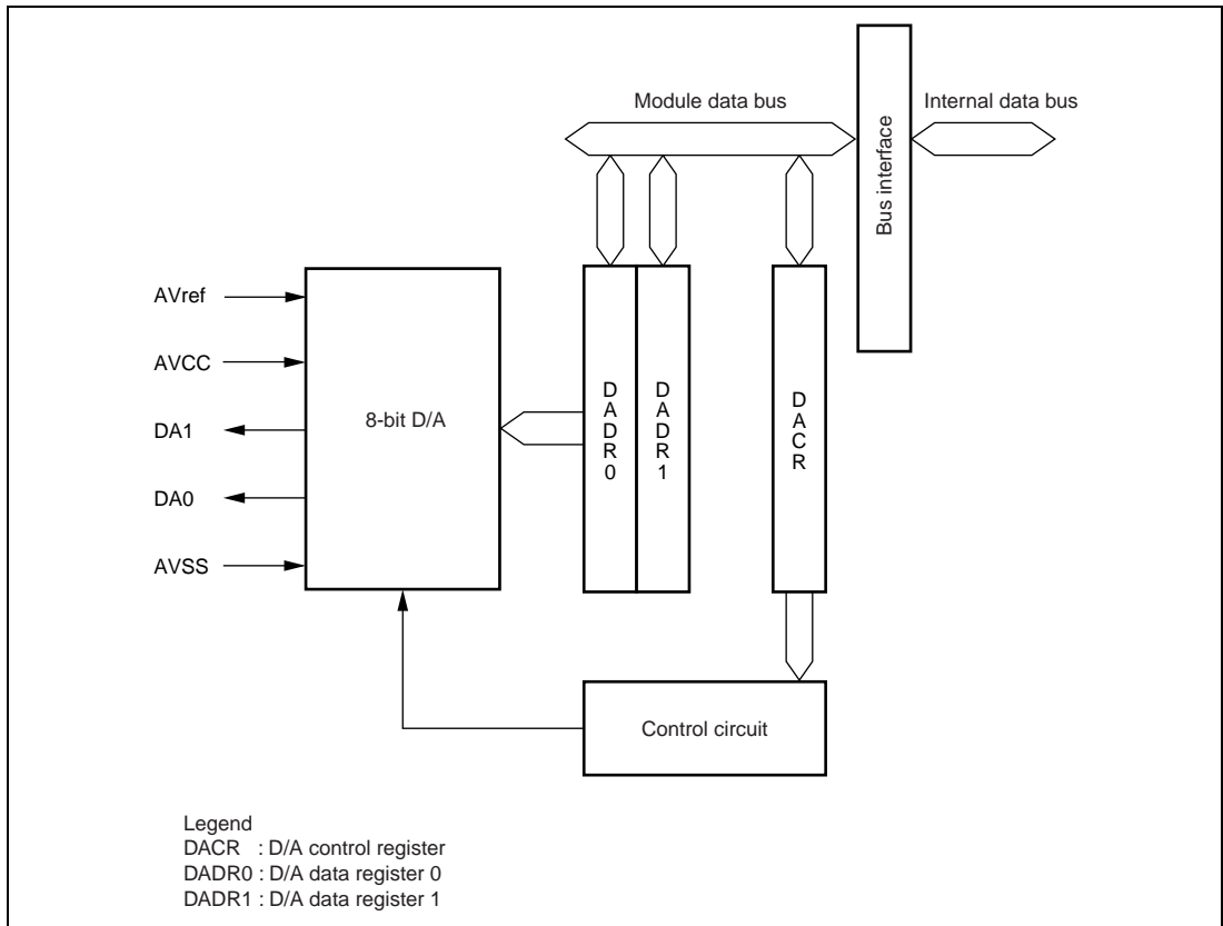
Figure 20.1 Block Diagram of D/A Converter
