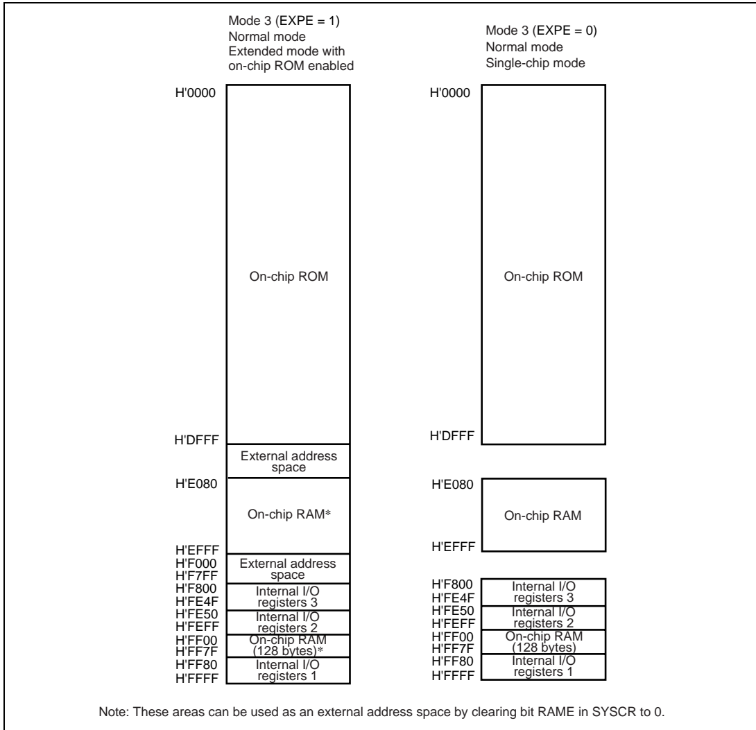
Figure 3.4 Address Map for H8S/2141B and H8S/2161B (2)
