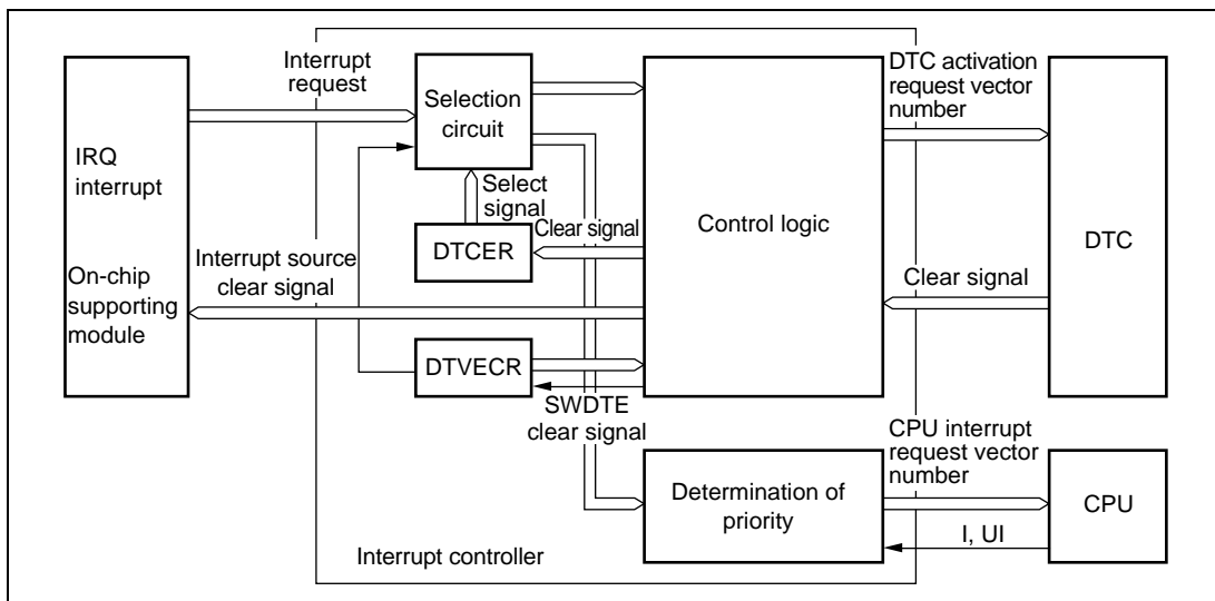
Figure 5.8 DTC and Interrupt Controller
