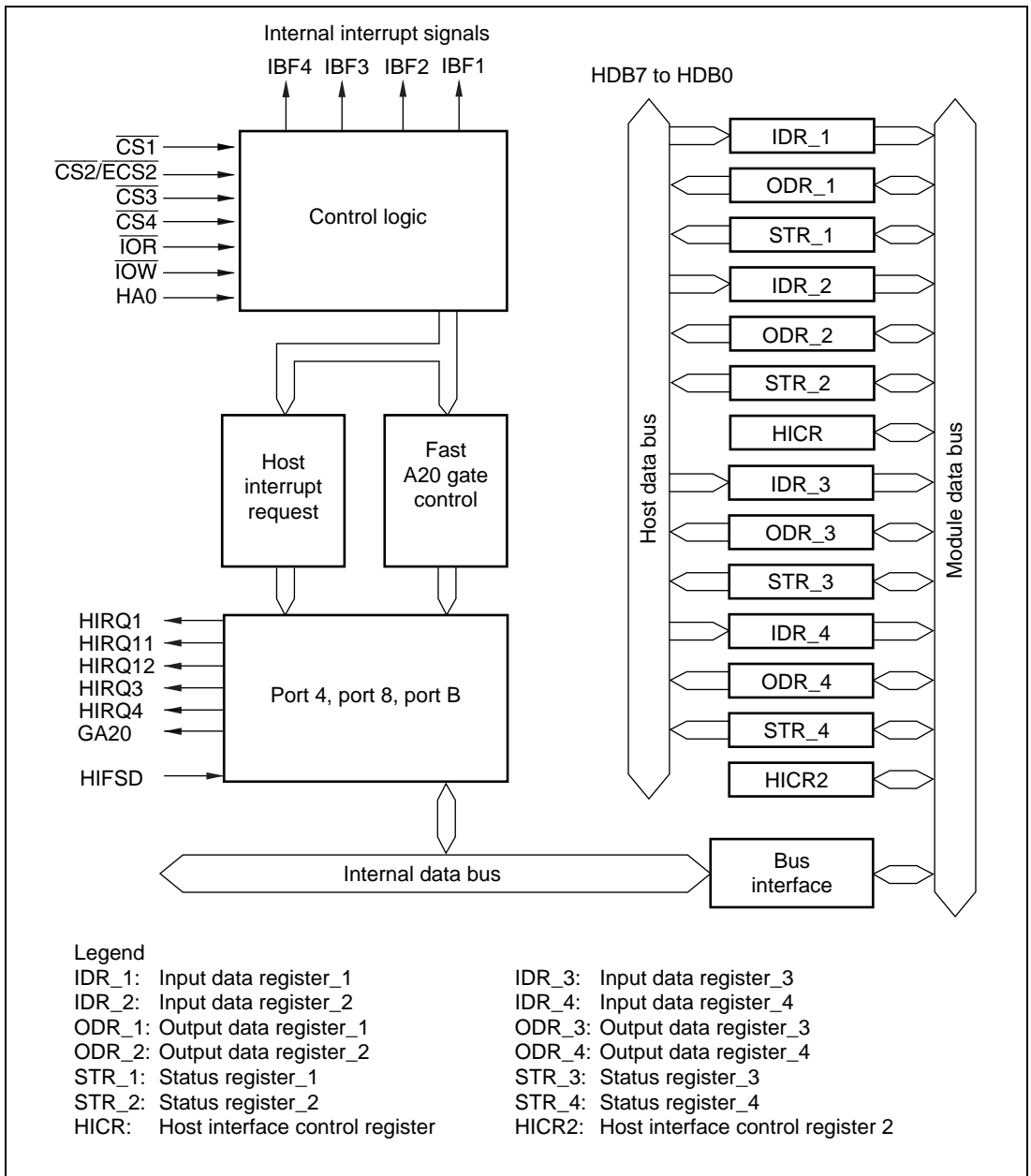
Figure 18.1 Block Diagram of XBS
