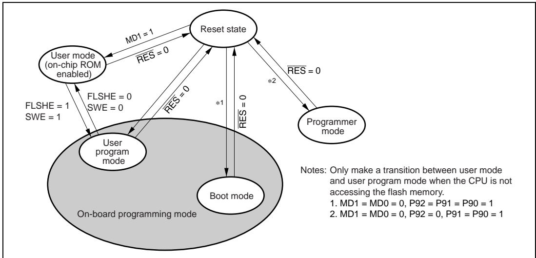
Figure 23.2 Flash Memory State Transitions
