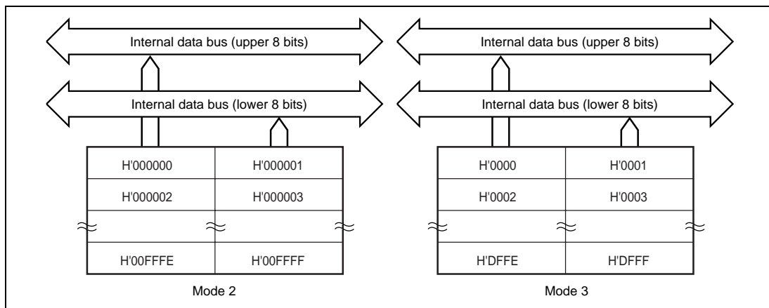
Figure 24.2 Block Diagram of 64-Kbyte Masked ROM (HD6432160BV)
