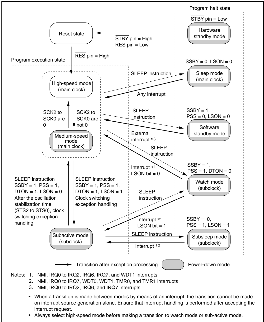
Figure 26.1 Mode Transition Diagram
