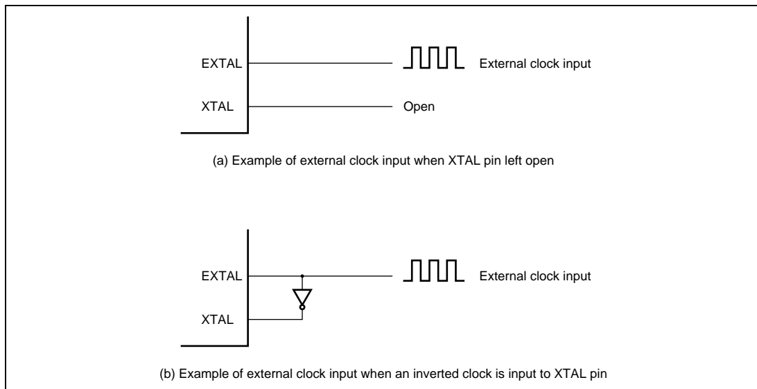
Figure 25.4 Example of External Clock Input
