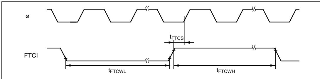
Figure 28.18 FRT Clock Input Timing
