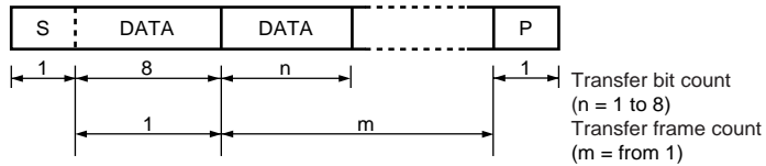
Figure 16.5 I 2 C Bus Data Format (Serial Format)
