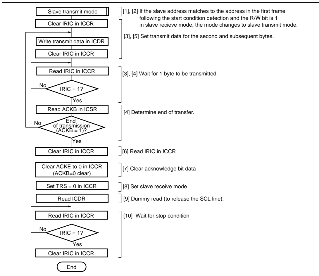
Figure 16.24 Sample Flowchart for Slave Transmit Mode
