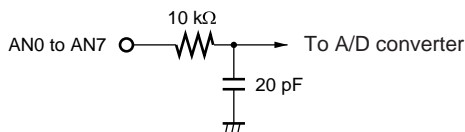
Figure 21.8 Example of Analog Input Protection Circuit
