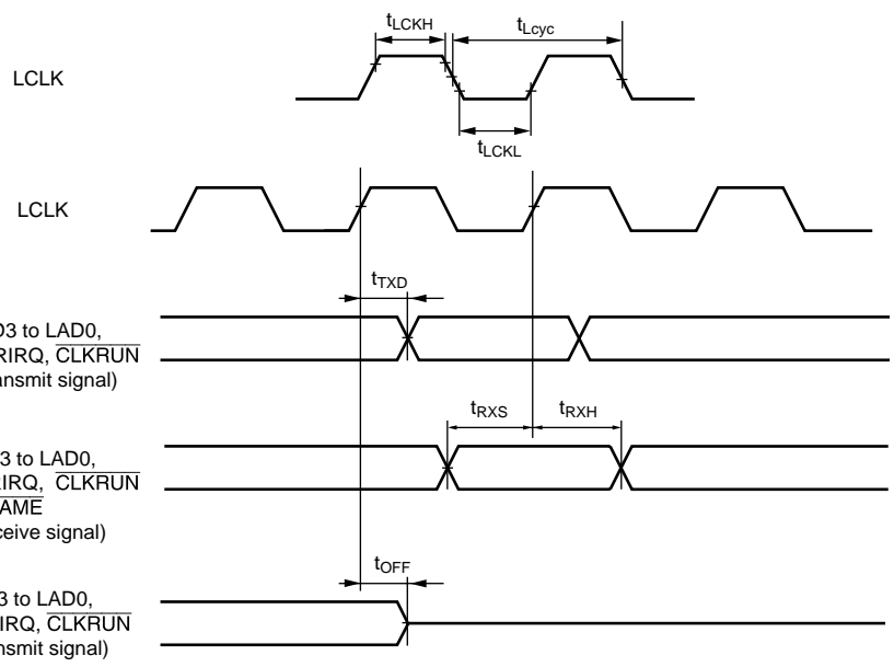
Figure 28.30 Host Interface (LPC) Timing
