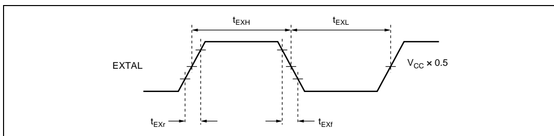
Figure 25.5 External Clock Input Timing
