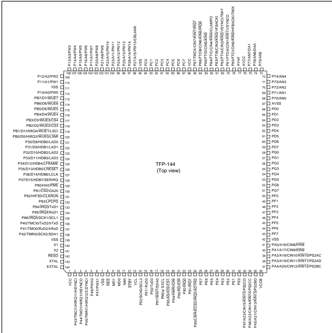
Figure 1.4 Pin Arrangement of H8S/2160B and H8S/2161B
