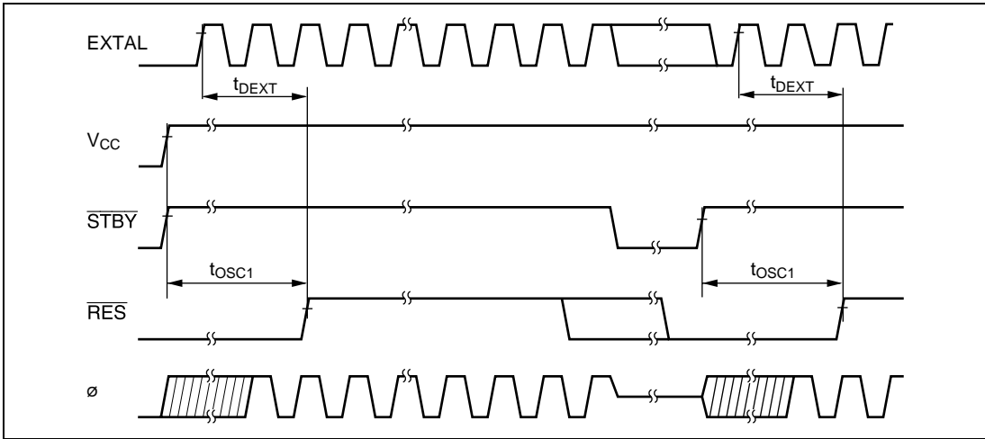
Figure 28.7 Oscillation Settling Timing
