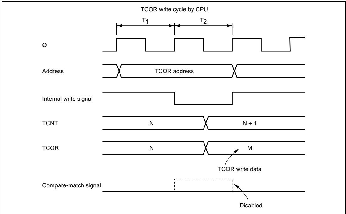
Figure 12.16 Conflict between TCOR Write and Compare-Match
