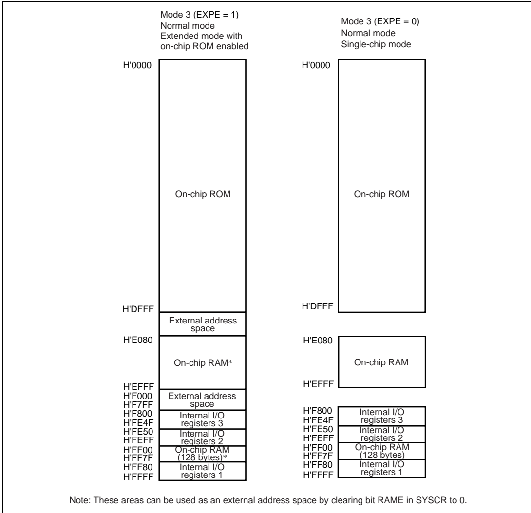
Figure 3.2 Address Map for H8S/2140B and H8S/2160B (2)
