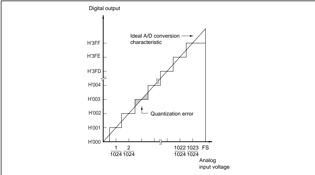
Figure 21.5 A/D Conversion Accuracy Definitions
