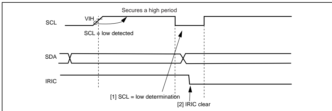
Figure 16.33 IRIC Flag Clearing Timing When WAIT = 1
