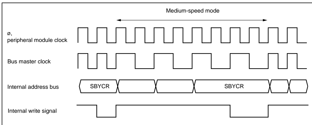
Figure 26.2 Medium-Speed Mode Timing
