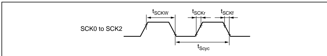
Figure 28.23 SCK Clock Input Timing
