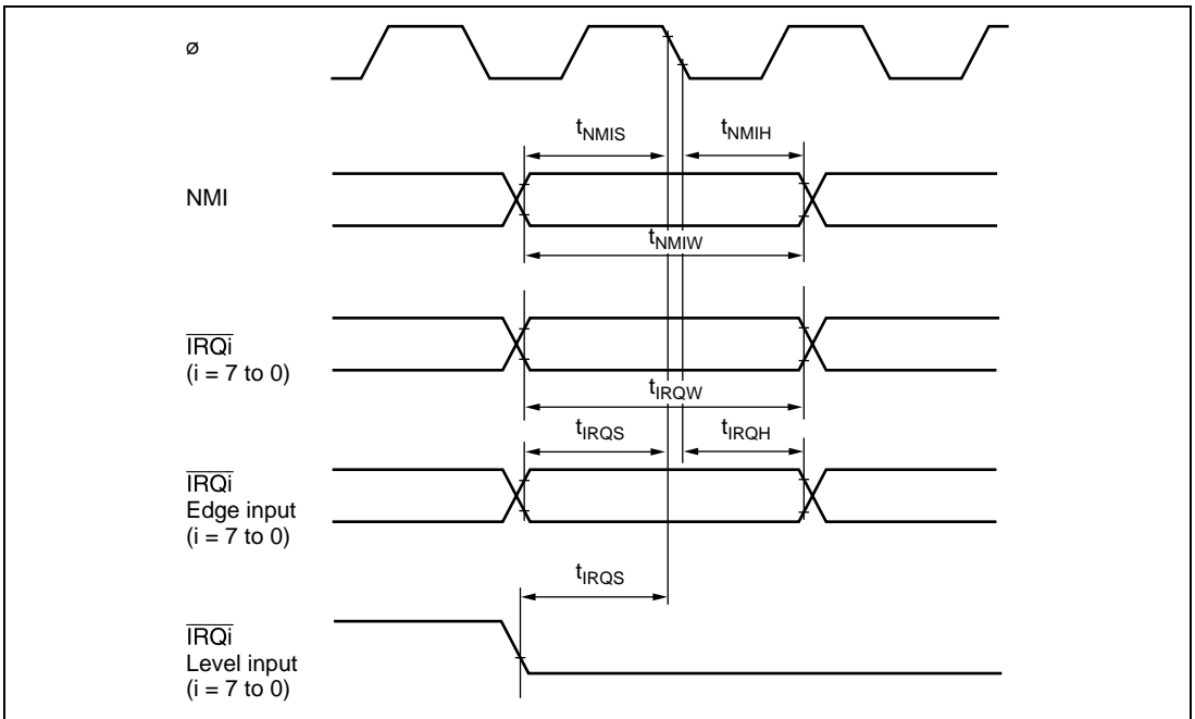
Figure 28.10 Interrupt Input Timing
