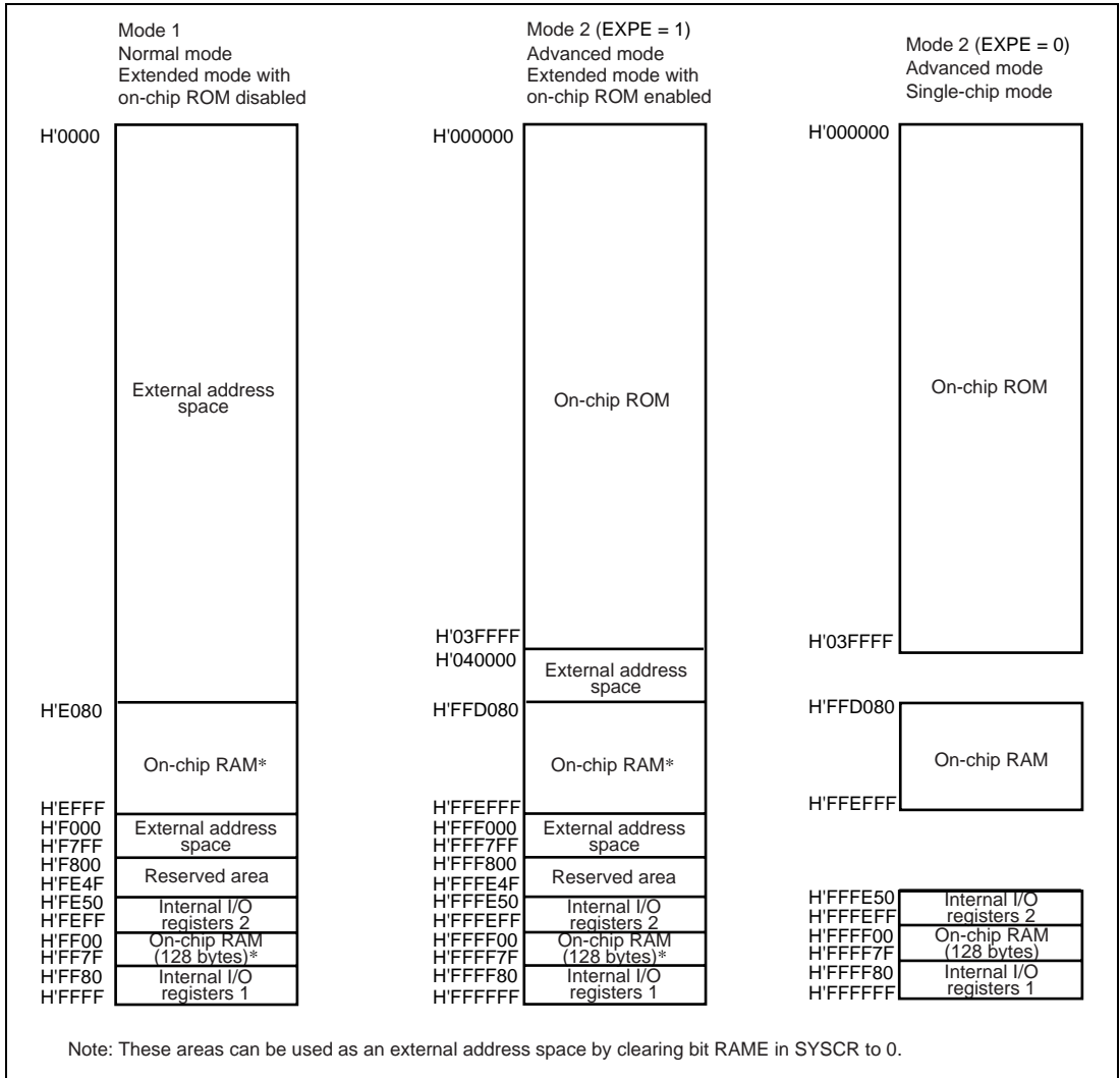
Figure 3.7 Address Map for H8S/2148B (1)
