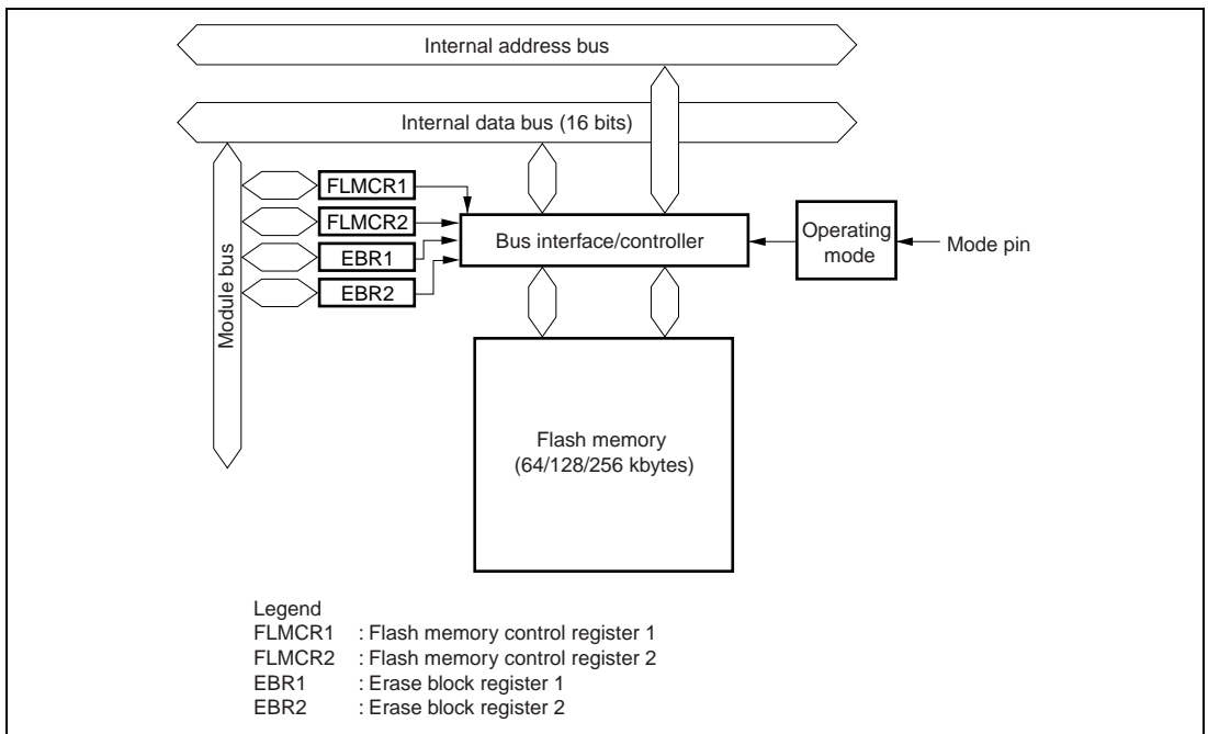
Figure 23.1 Block Diagram of Flash Memory
