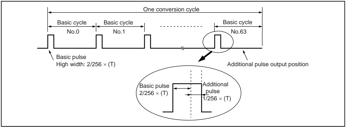
Figure 10.6 Output Waveform when DADR = H'0207 ( OS = 1 )
