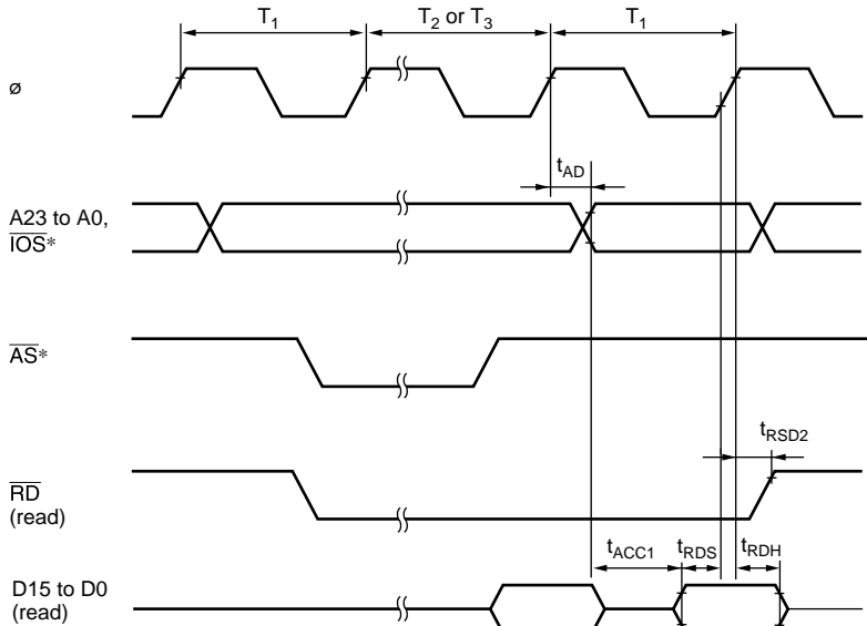
Figure 28.14 Burst ROM Access Timing (Two-State Access)
