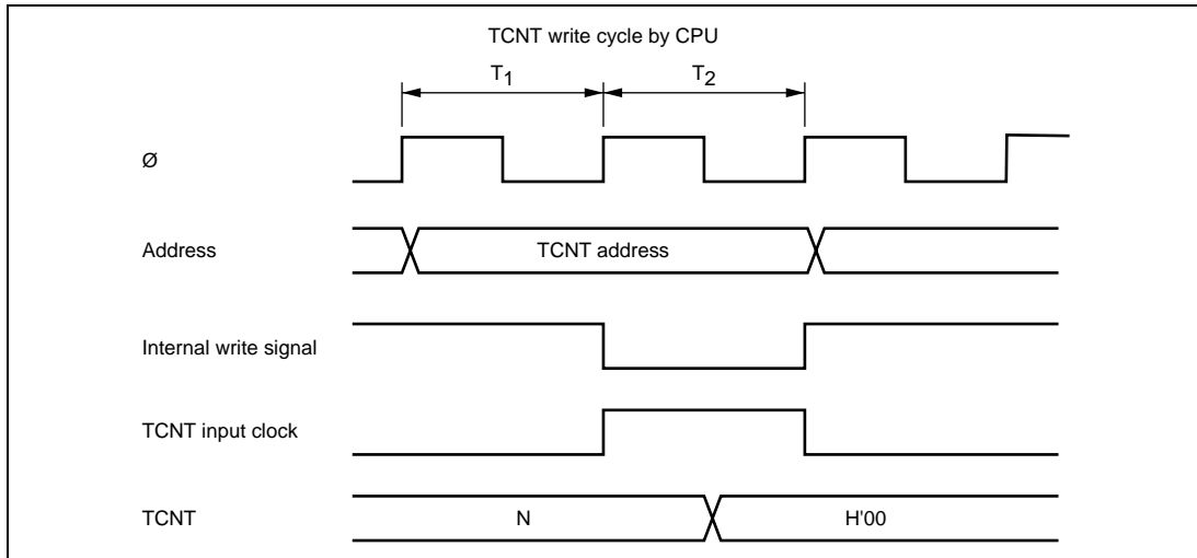
Figure 12.14 Conflict between TCNT Write and Clear
