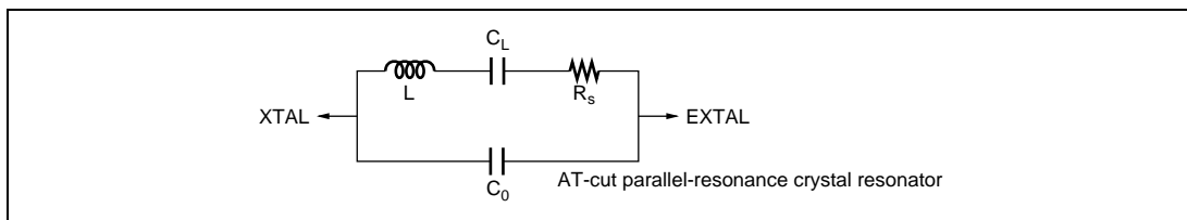
Figure 25.3 Equivalent Circuit of Crystal Resonator
