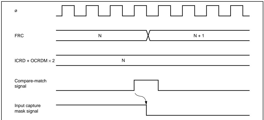
Figure 11.16 Timing of Input Capture Mask Signal Clearing
