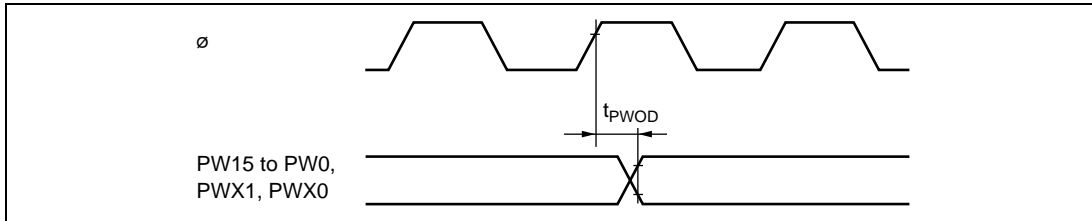
Figure 28.22 PWM, PWMX Output Timing
