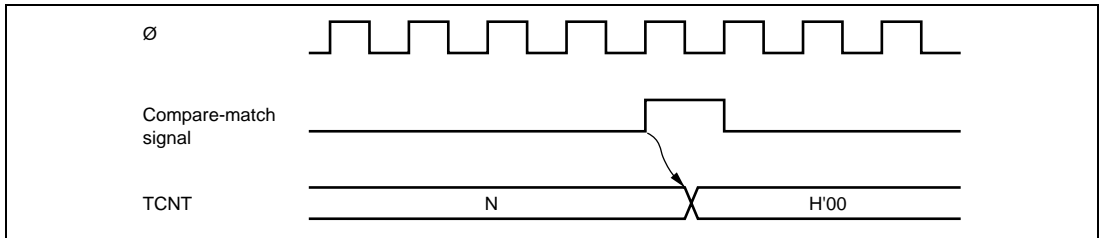
Figure 12.8 Timing of Counter Clear by Compare-Match
