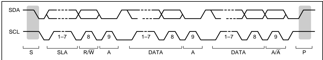
Figure 16.6 I 2 C Bus Timing
