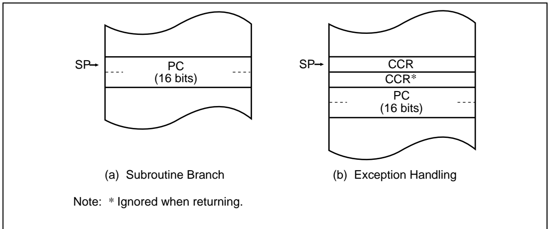
Figure 2.2 Stack Structure in Normal Mode
