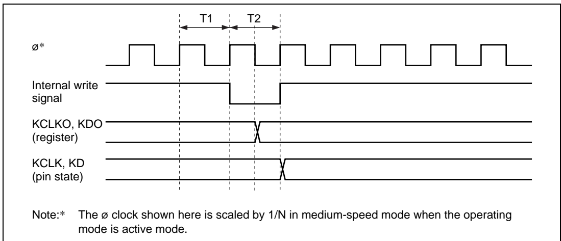
Figure 17.10 KCLKO and KDO Write Timing
