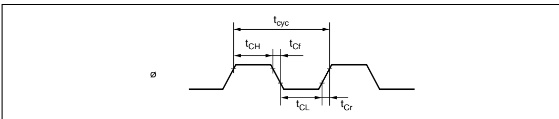
Figure 28.6 System Clock Timing
