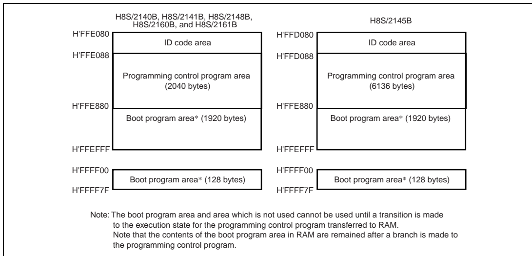
Figure 23.8 On-Chip RAM Area in Boot Mode
