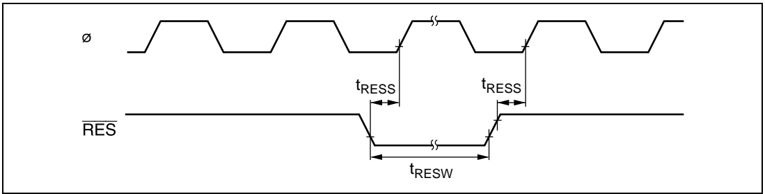
Figure 28.9 Reset Input Timing
