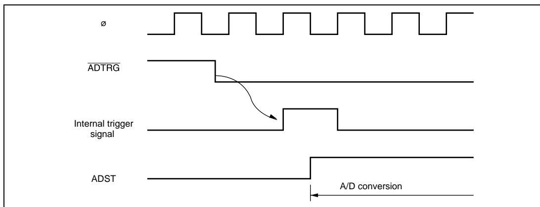
Figure 21.4 External Trigger Input Timing
