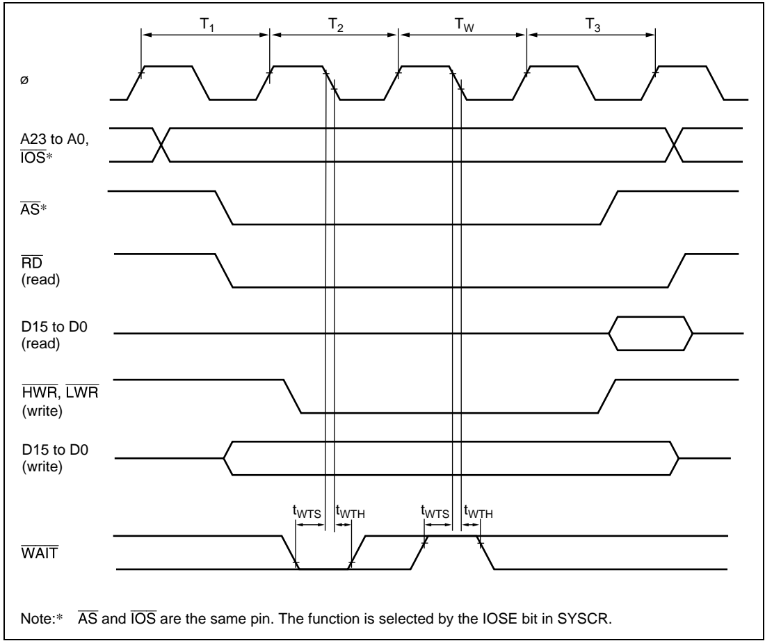
Figure 28.13 Basic Bus Timing (Three-State Access with One Wait State)
