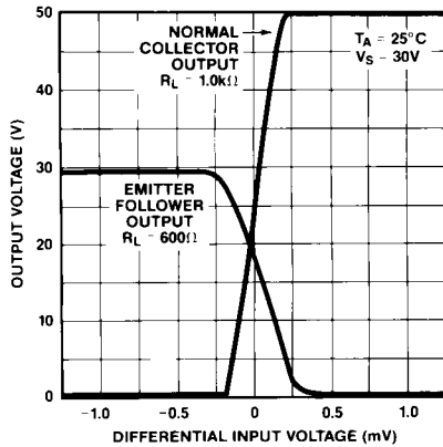
TRANSFER FUNCTION
