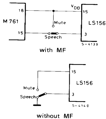
Fig. 10 – External mute function
