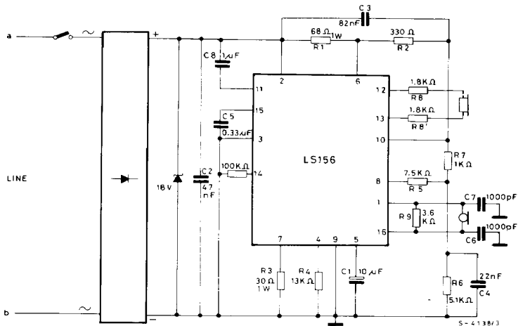
Fig. 11 – Application circuit without multifrequency.
